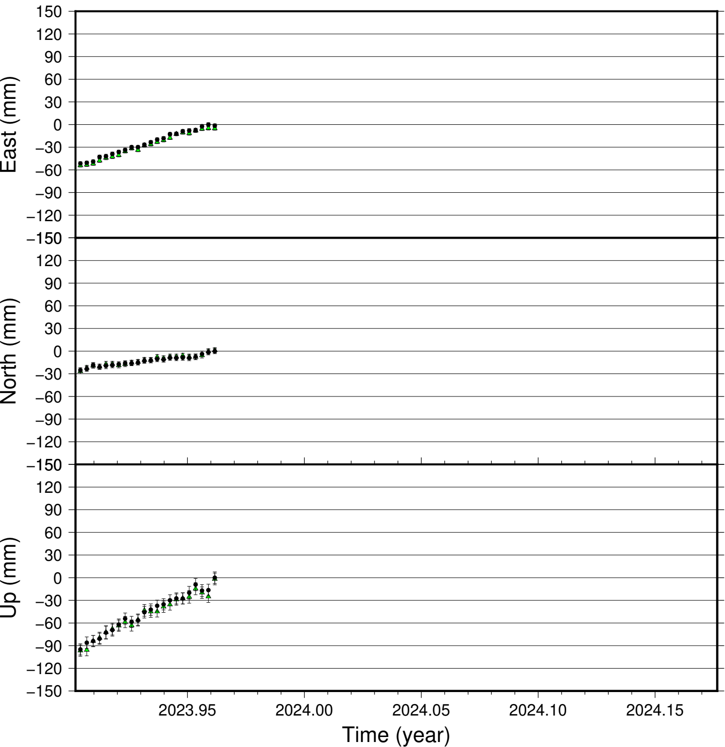
SUND time series (IGS 2014), last 100 days
