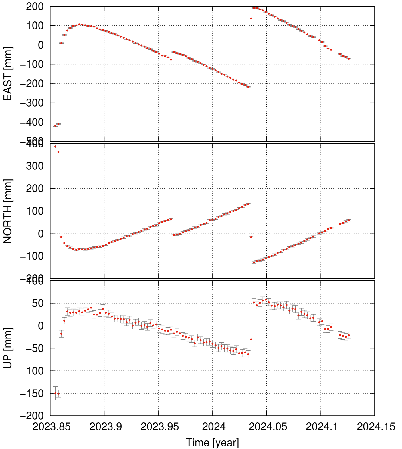
SUDV residual time series (some major events removed as well)
