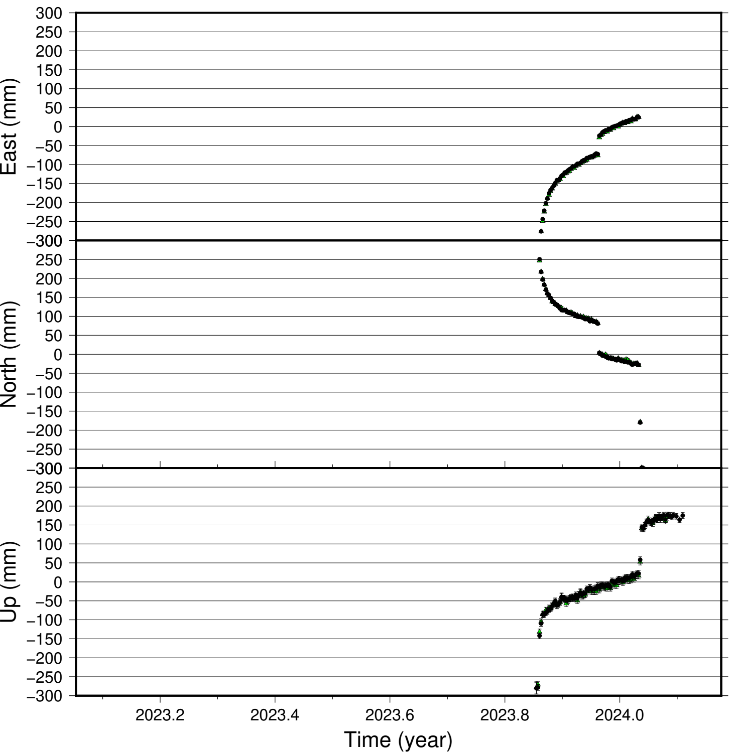
SUDV time series (IGS 2014), last 400 days
