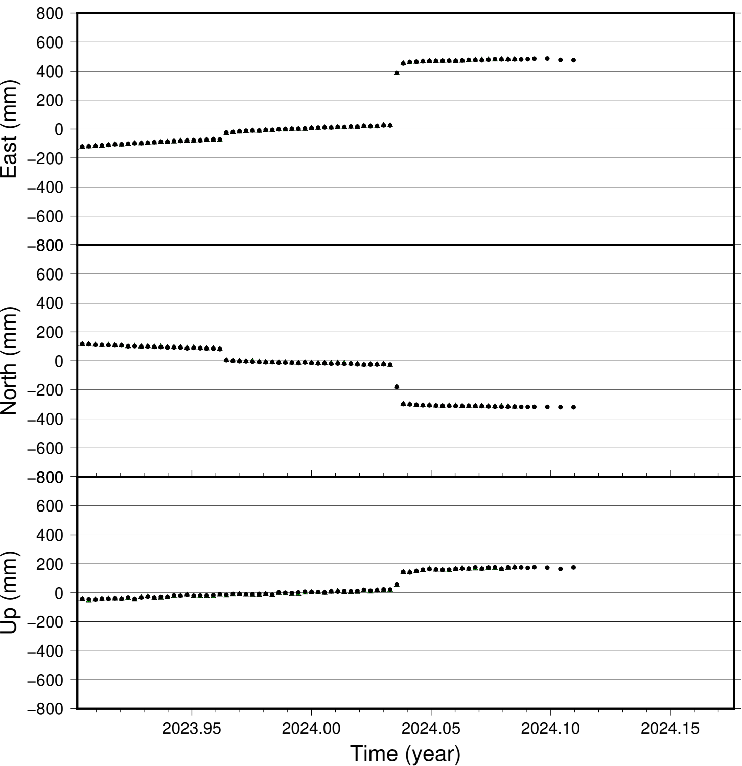
SUDV time series (IGS 2014), last 100 days
