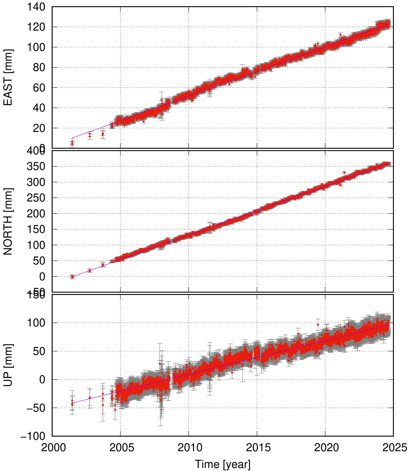
STOR (63.75, -20.21) time series (ITRF 2014) v_e = 4.86 \pm 0.10 ; v_n = 15.52 \pm 0.15 ; v_u = 5.93 \pm 0.27 mm/yr
