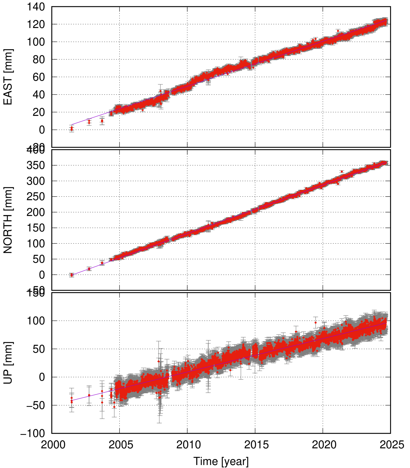
STOR (63.75, -20.21) time series (ITRF 2014) v_e = 5.10 \pm 0.13 ; v_n = 15.52 \pm 0.15 ; v_u = 5.93 \pm 0.27 mm/yr
