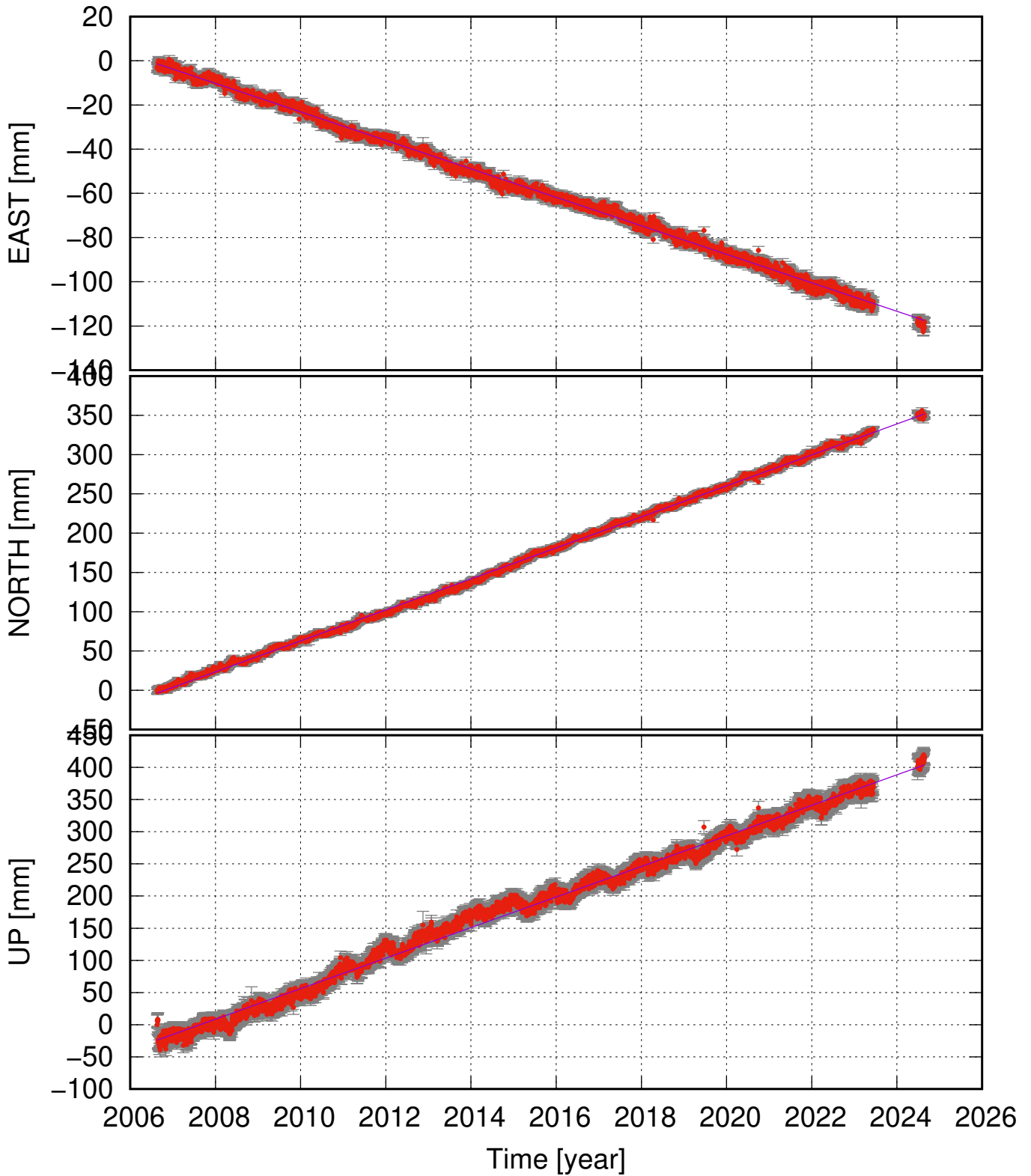
STKA (64.44, -18.82) time series (ITRF 2014) v_e = -6.45 \pm 0.09 ; v_n = 19.72 \pm 0.16 ; v_u = 23.76 \pm 0.54 mm/yr
