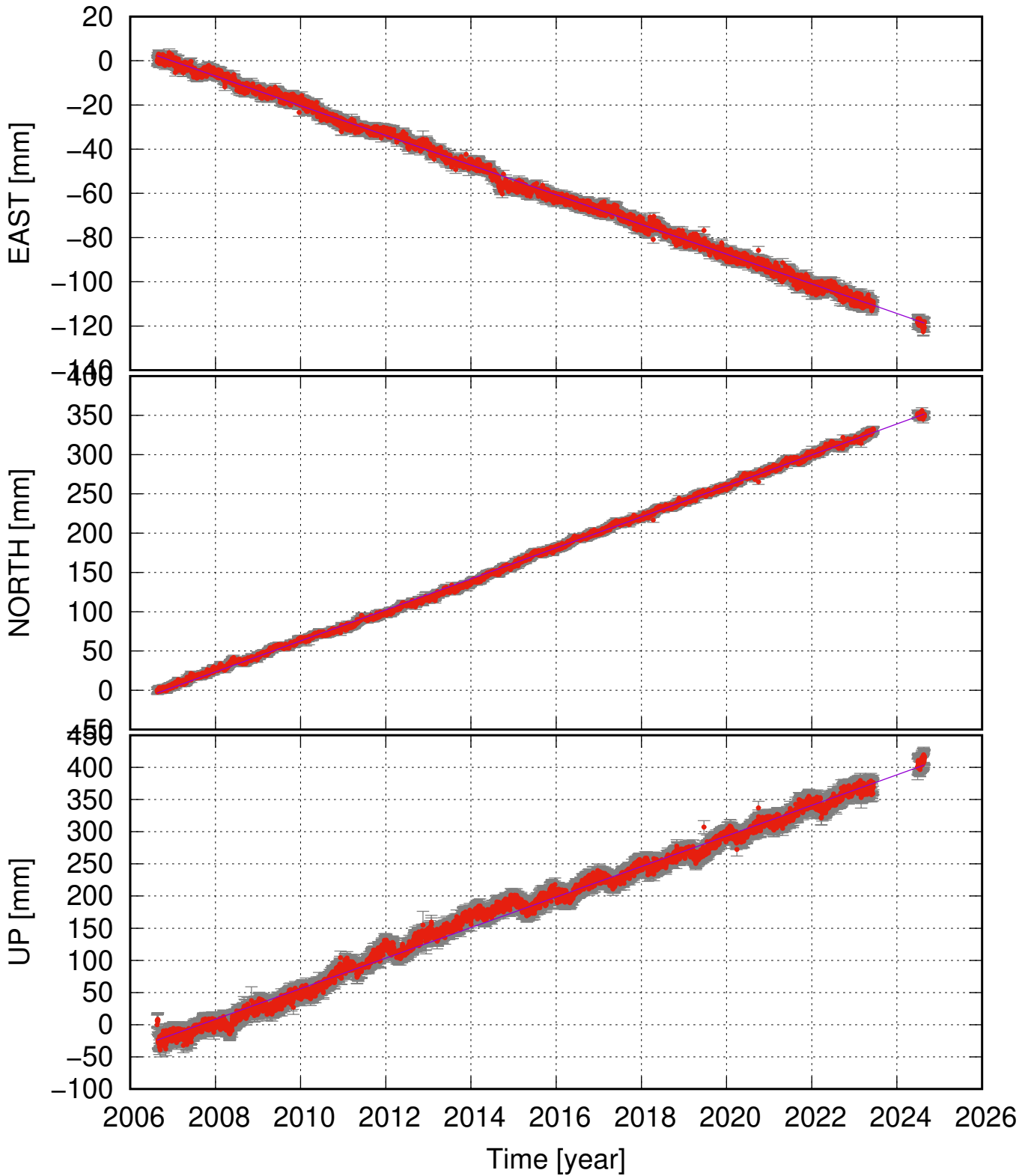
STKA (64.44, -18.82) time series (ITRF 2014) v_e = -6.72 \pm 0.09 ; v_n = 19.72 \pm 0.16 ; v_u = 23.76 \pm 0.54 mm/yr
