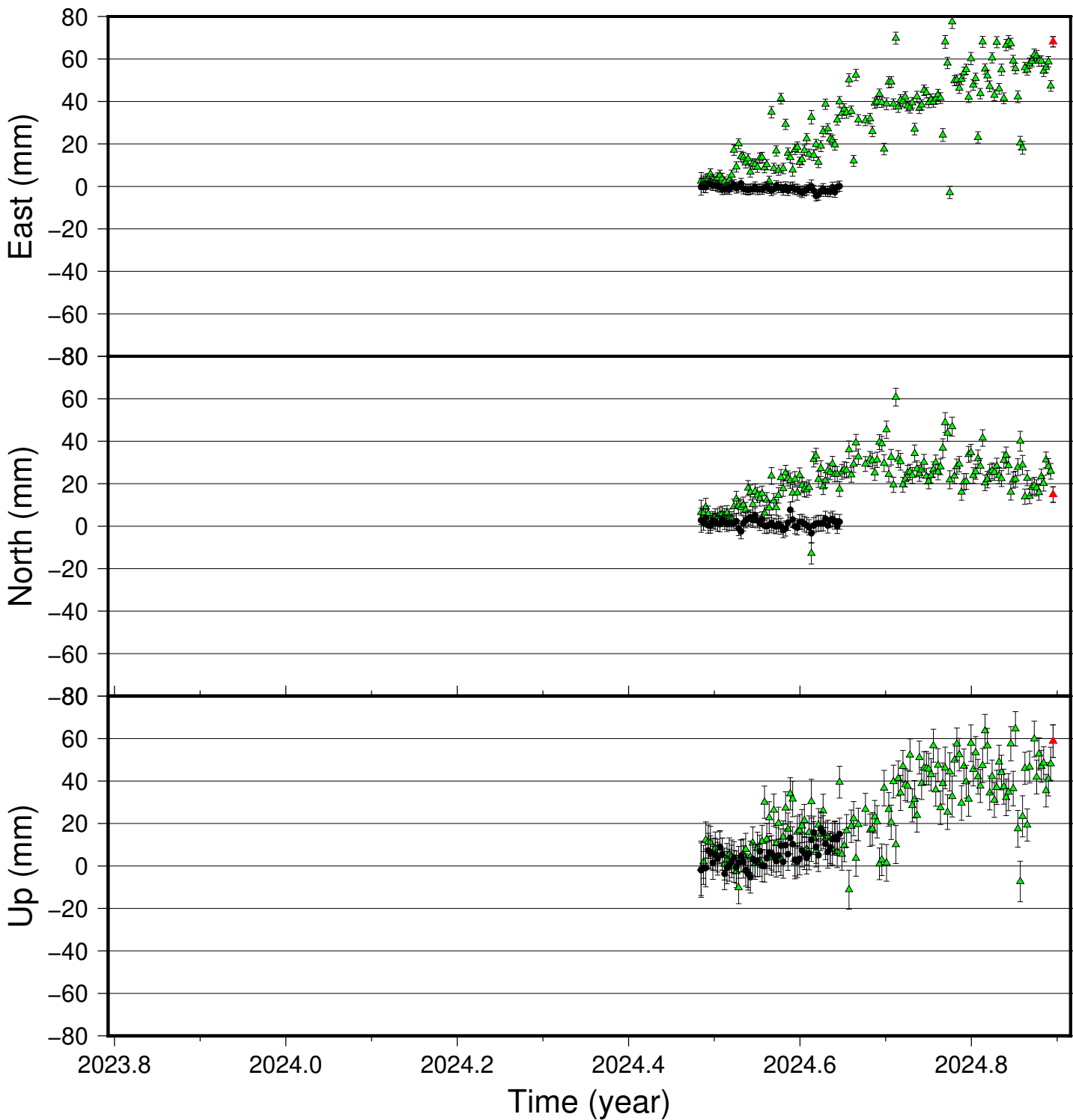
STKA time series (IGS 2014), last 400 days
