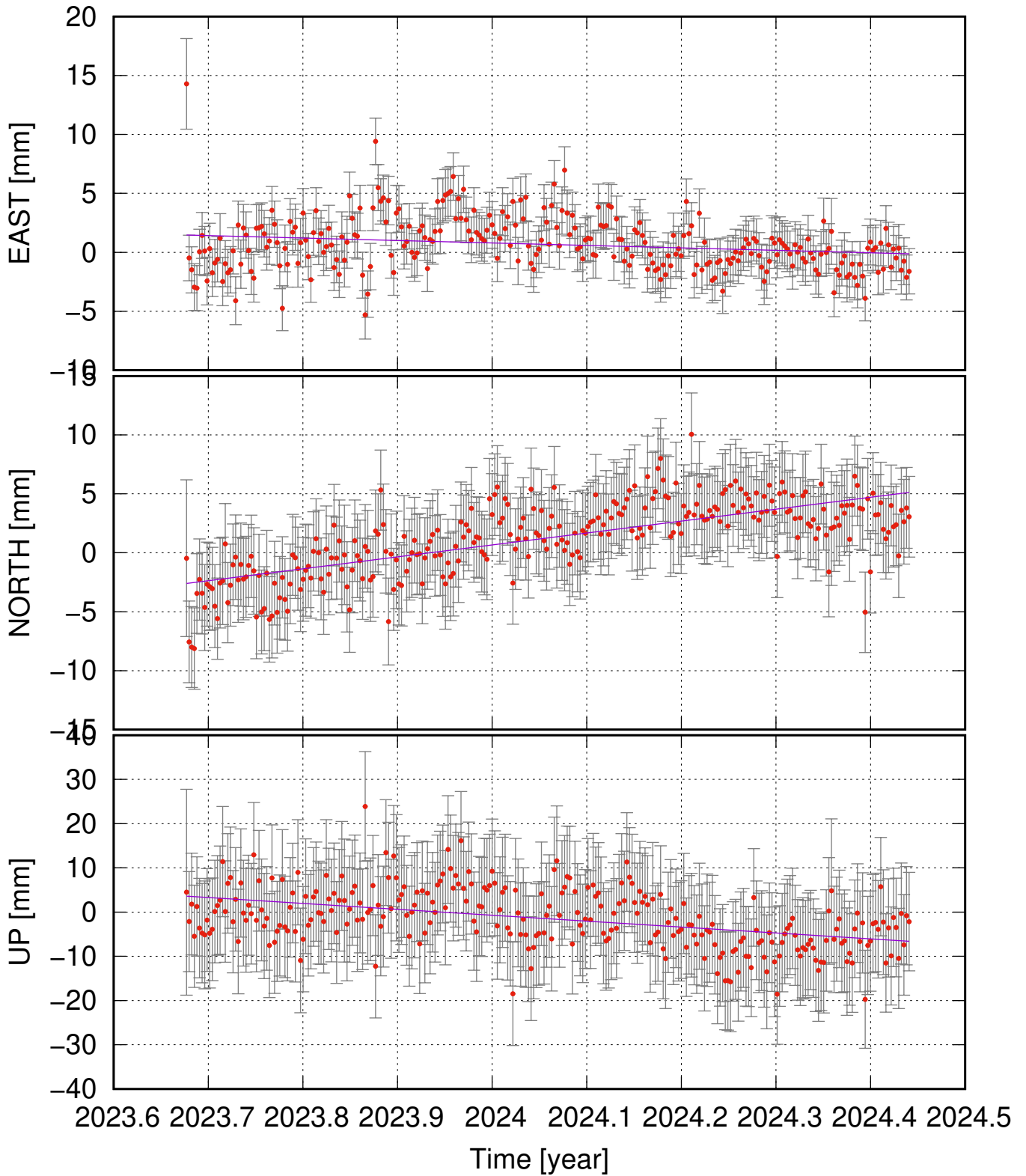
STHV (63.96, -19.15) time series (ITRF 2014) ve = -2.09 \pm 2.95 ; vn = 10.12 \pm 2.86 ; vu = -13.35 \pm 7.78 mm/yr
