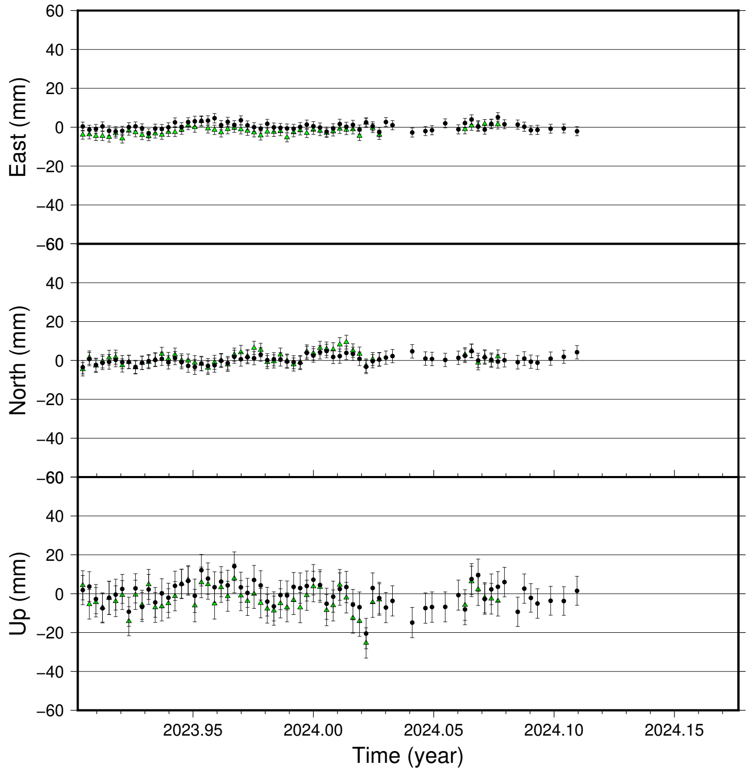
STHV time series (IGS 2014), last 100 days
