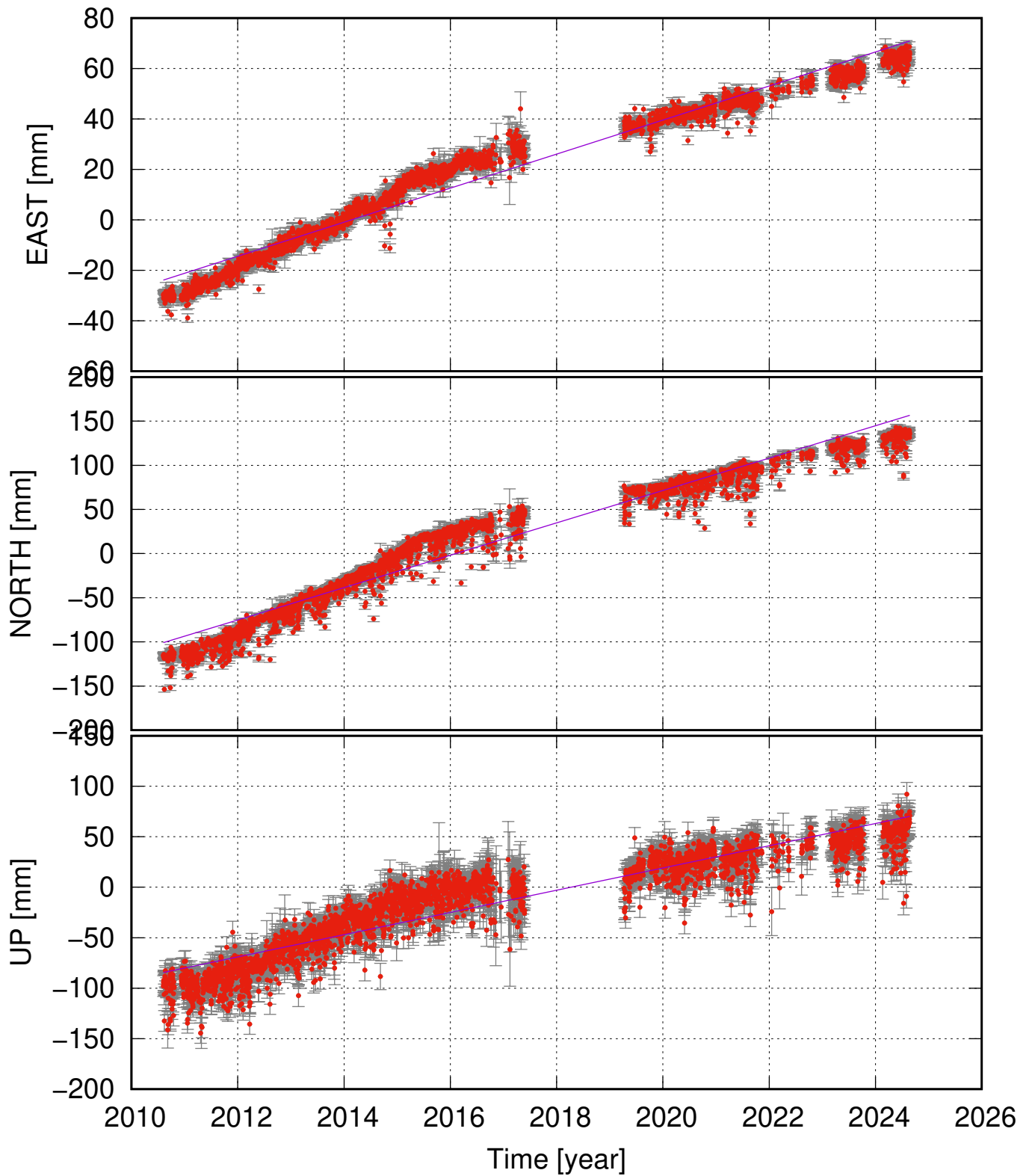
STE2 (63.68, -19.61) time series (ITRF 2014) v_e = 6.74 \pm 0.38 ; v_n = 18.33 \pm 1.20 ; v_u = 11.01 \pm 1.28 mm/yr
