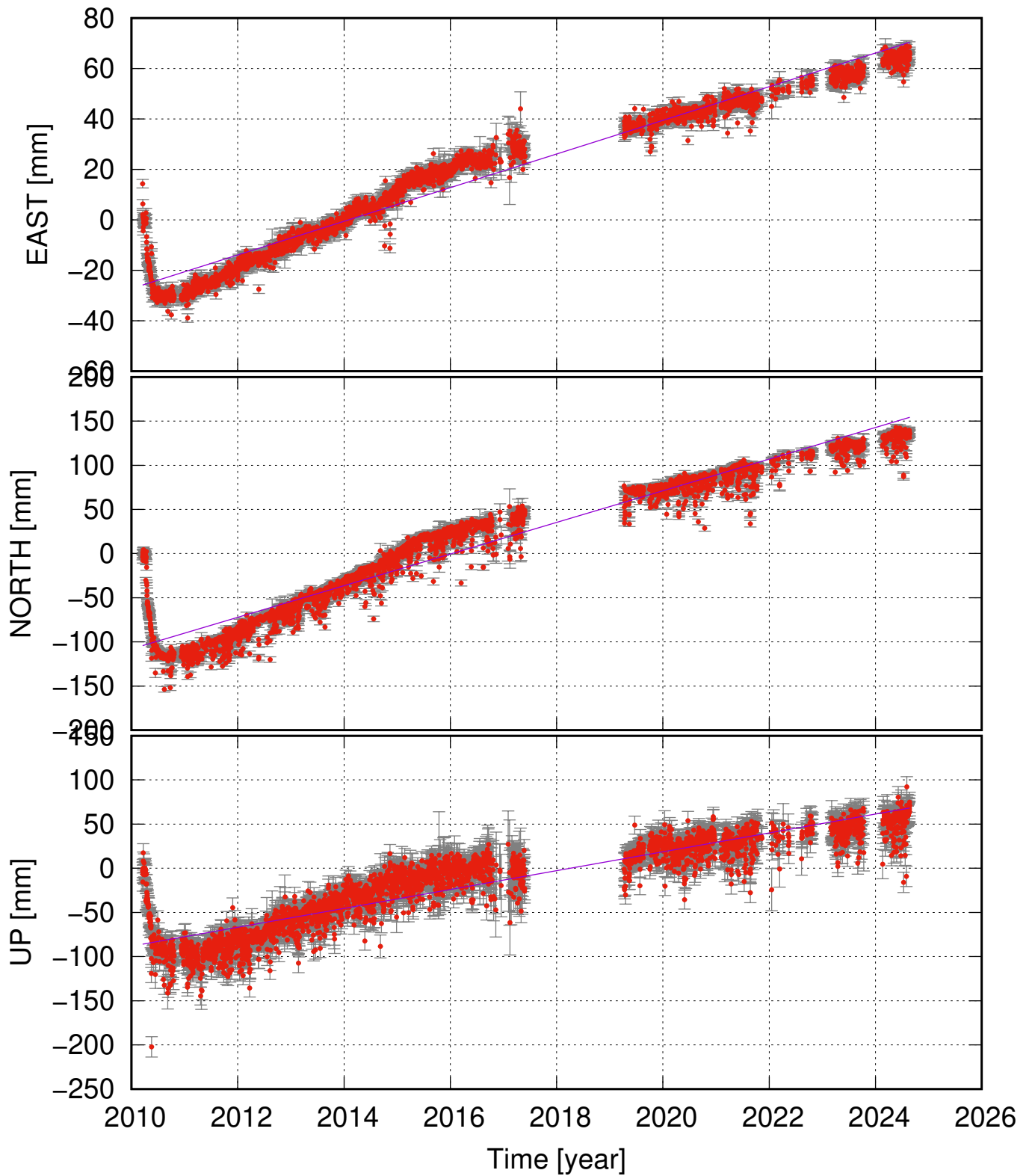
STE2 (63.68, -19.61) time series (ITRF 2014) v_e = 6.67 \pm 0.40 ; v_n = 17.91 \pm 1.34 ; v_u = 10.68 \pm 1.35 mm/yr
