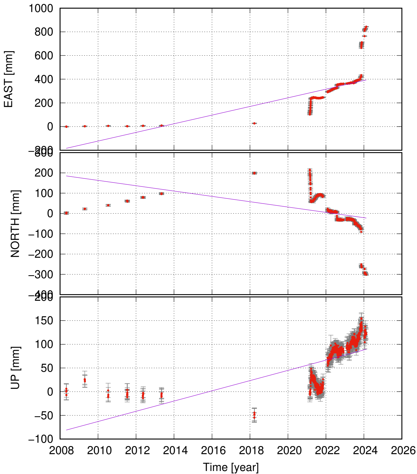
STAN (63.85, -22.23) time series (ITRF 2014) ve = 36.54 ± 5.79; vn = -13.14 ± 4.77; vu = 10.78 ± 2.20 mm/yr
