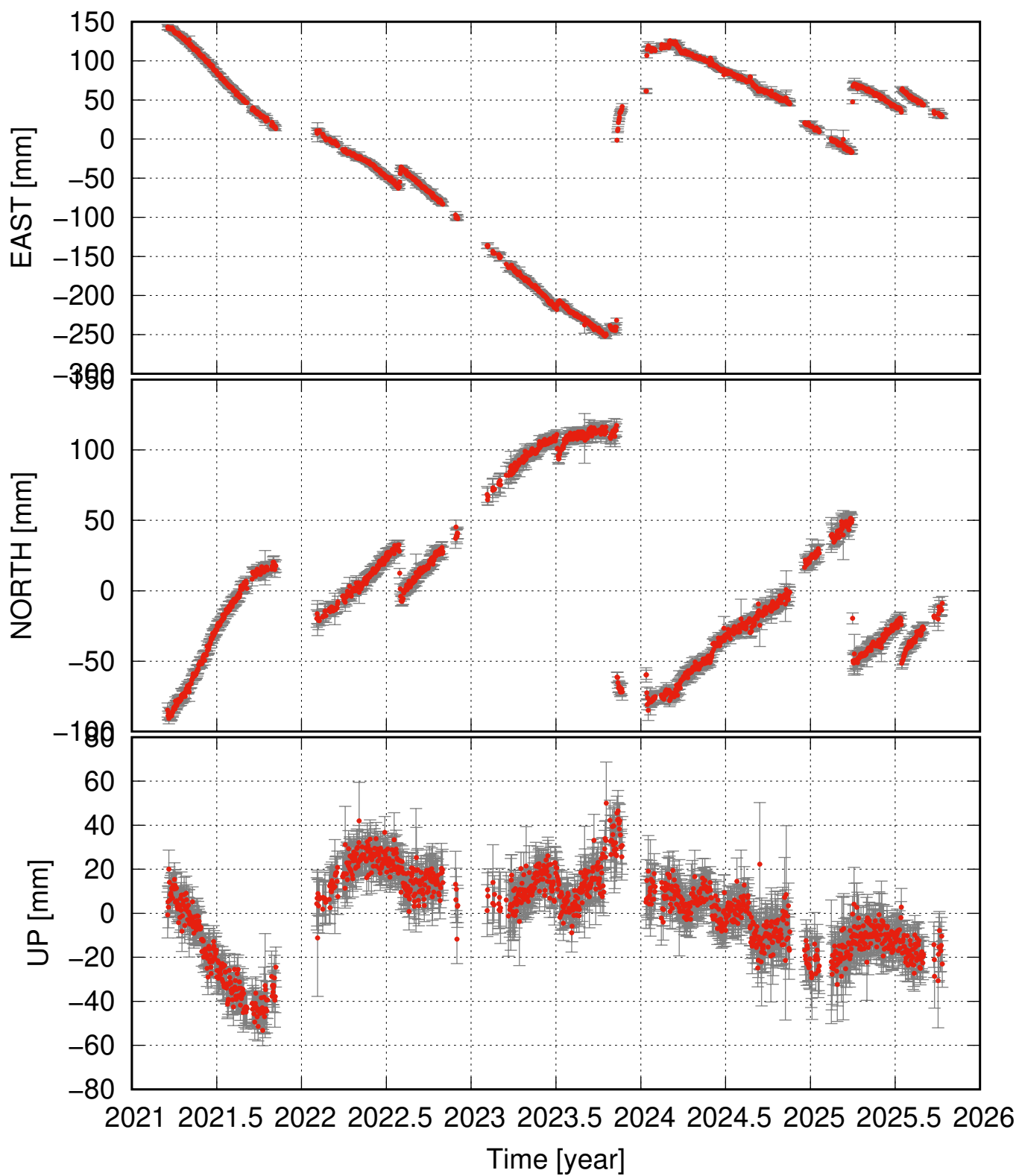
STAN residual time series
