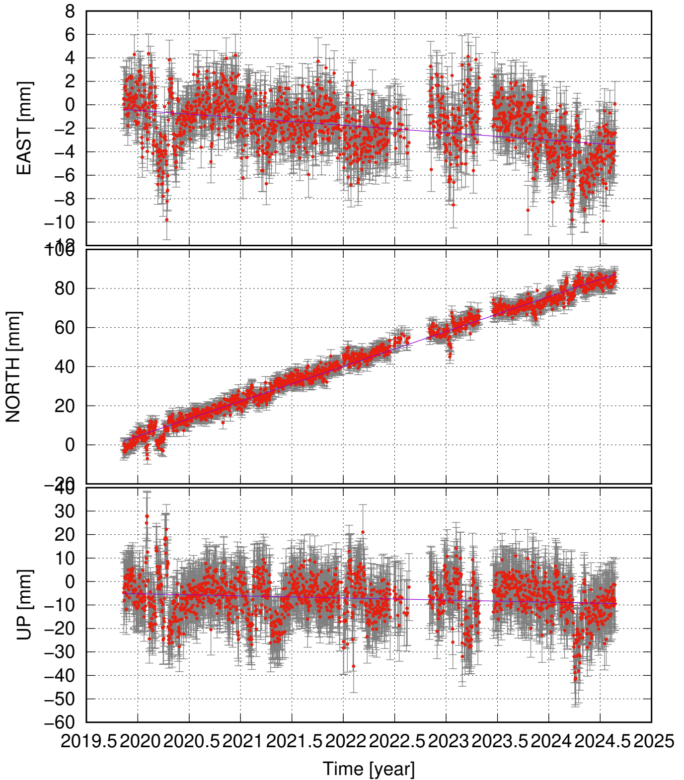
SPBC (65.72, -16.75) time series (ITRF 2014) v_e = -0.63 \pm 0.44 ; v_n = 17.84 \pm 0.61 ; v_u = -0.91 \pm 1.79 mm/yr
