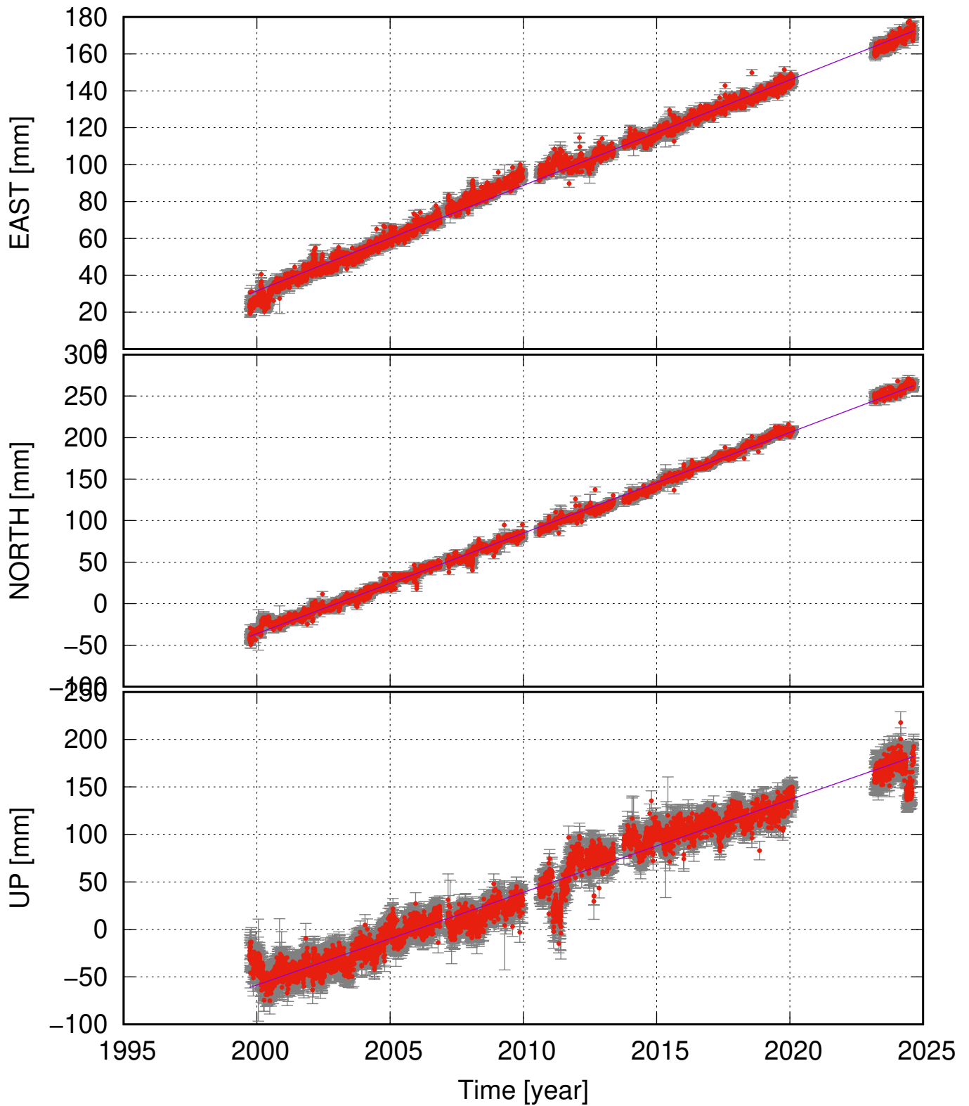
SOHO (63.55, -19.25) time series (ITRF 2014) v_e = 5.72 \pm 0.12 ; v_n = 12.12 \pm 0.16 ; v_u = 9.76 \pm 0.46 mm/yr
