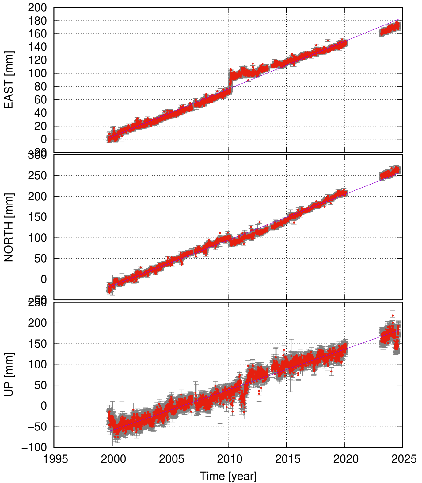
SOHO (63.55, -19.25) time series (ITRF 2014) v_e = 7.22 \pm 0.26 ; v_n = 11.01 \pm 0.26 ; v_u = 9.77 \pm 0.46 mm/yr
