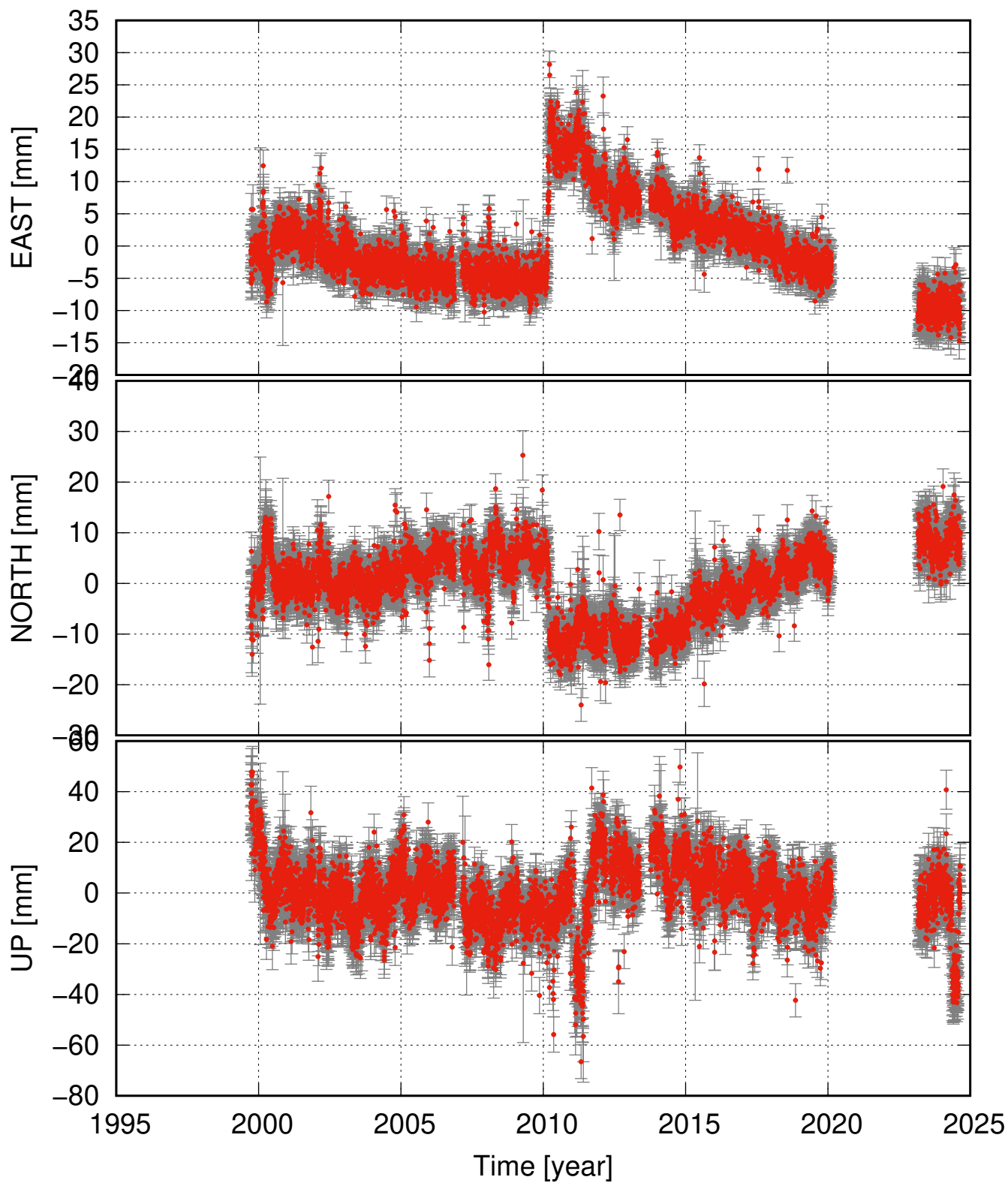
SOHO residual time series
