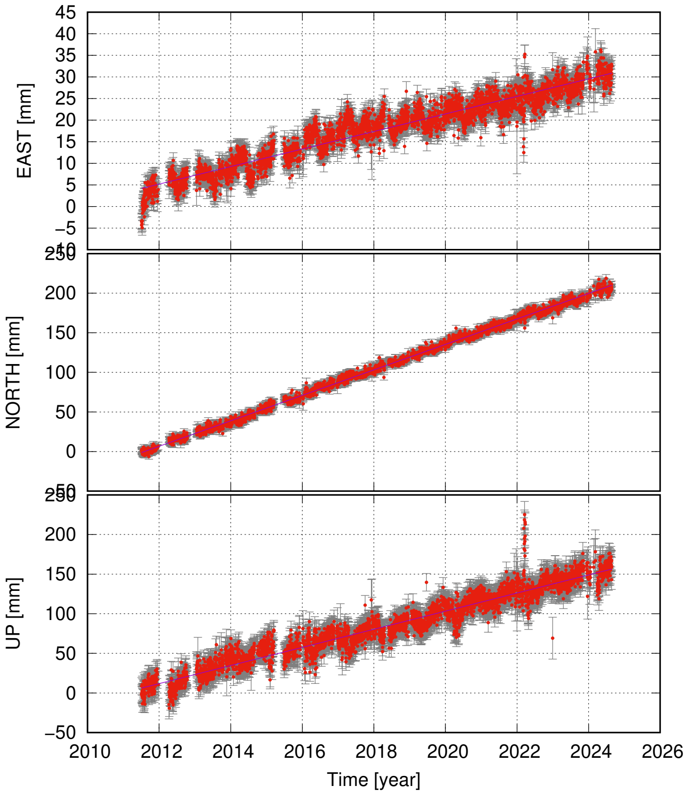
SODU (63.96, -19.59) time series (ITRF 2014) v_e = 2.03 \pm 0.17 ; v_n = 16.07 \pm 0.26 ; v_u = 11.43 \pm 0.82 mm/yr
