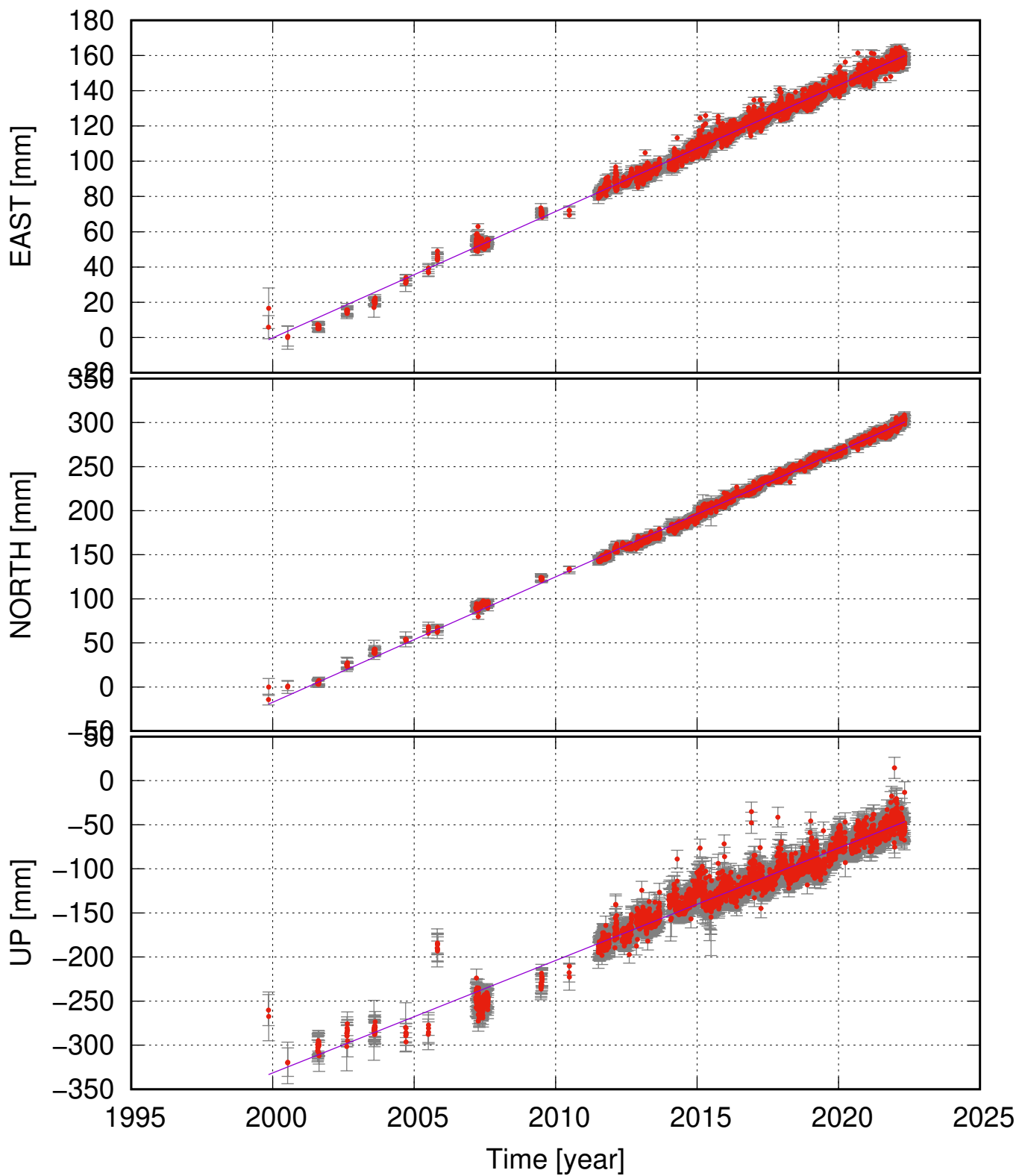
SNAE (63.74, -18.63) time series (ITRF 2014) v_e = 7.17 \pm 0.12 ; v_n = 14.24 \pm 0.14 ; v_u = 12.76 \pm 0.48 mm/yr
