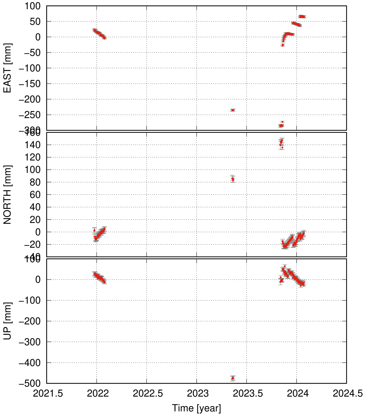
SLEI residual time series (some major events removed as well)
