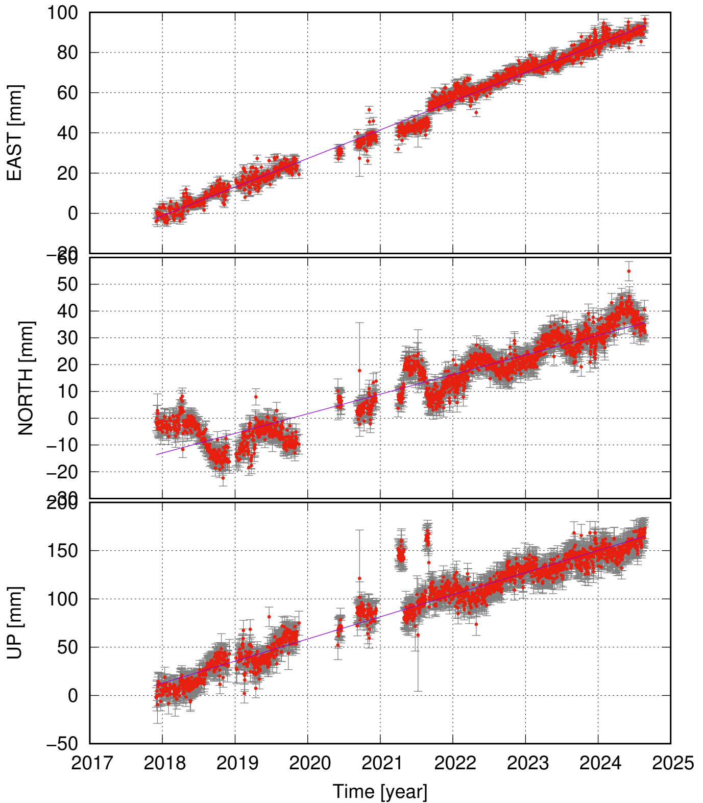
SLEC (63.94, -16.63) time series (ITRF 2014) v_e = 14.25 \pm 0.44 ; v_n = 7.32 \pm 0.81 ; v_u = 22.92 \pm 1.93 mm/yr
