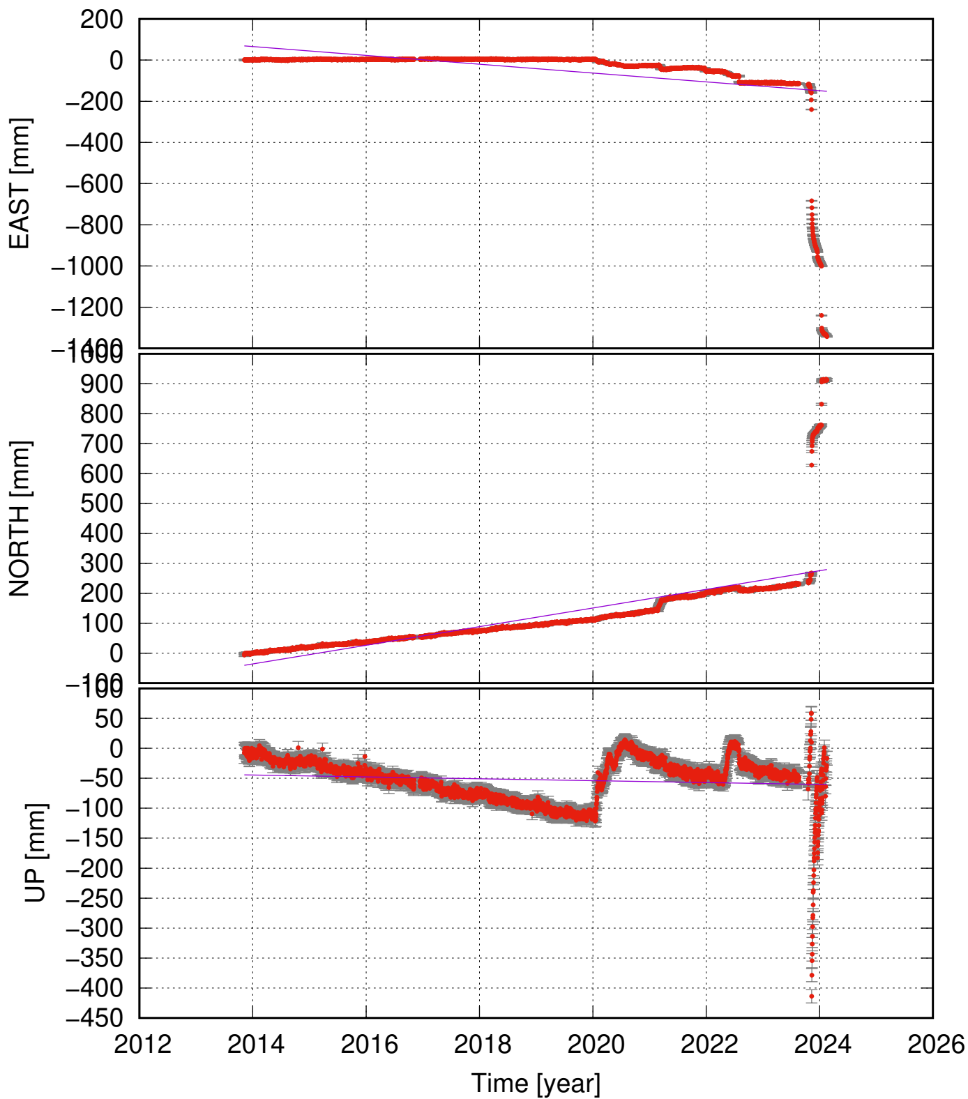
SKSH (63.87, -22.48) time series (ITRF 2014) v_e = -21.45 \pm 14.37 ; v_n = 31.15 \pm 8.27 ; v_u = -1.57 \pm 3.51 mm/yr
