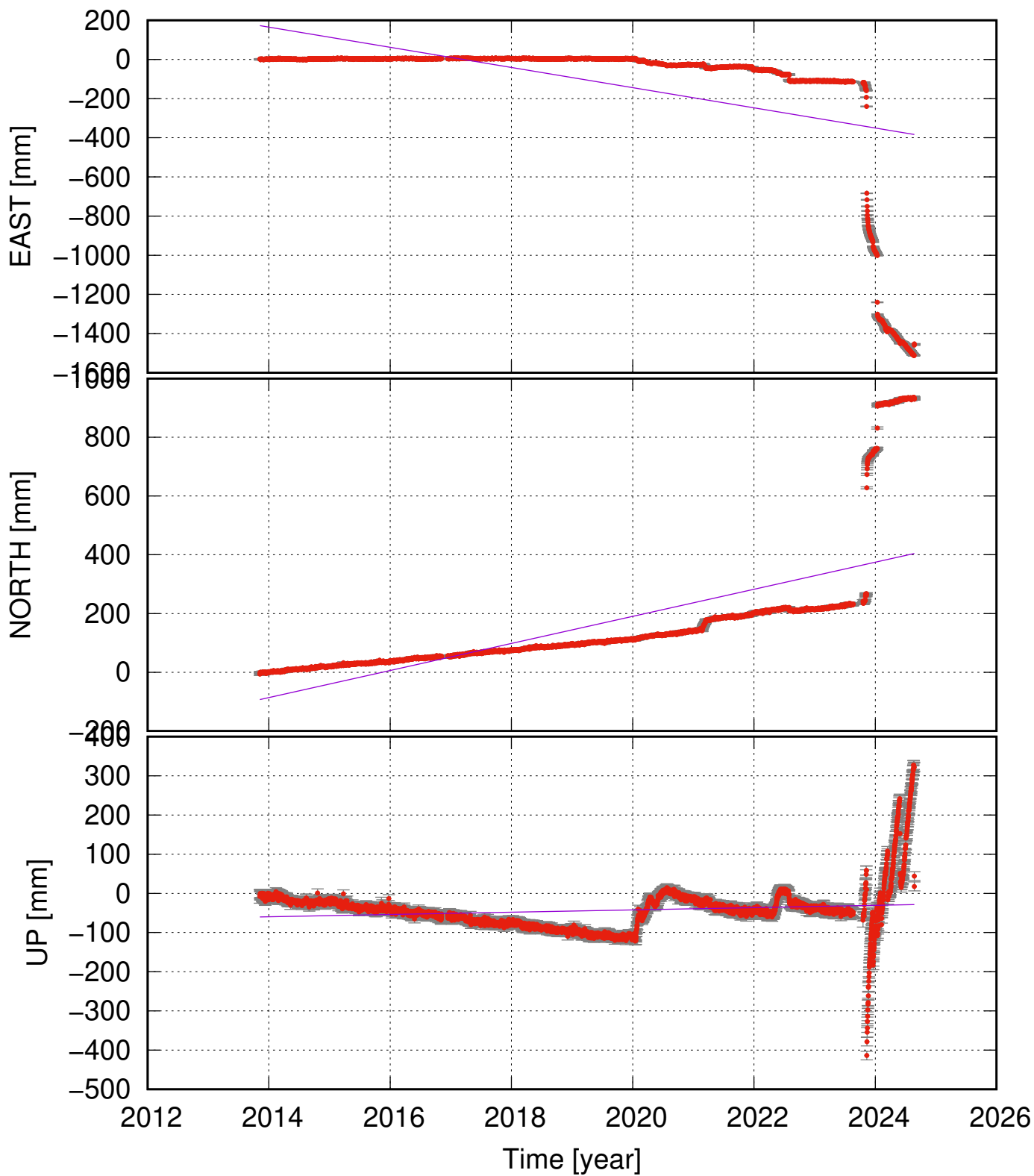
SKSH (63.87, -22.48) time series (ITRF 2014) v_e = -51.51 \pm 26.98 ; v_n = 46.07 \pm 14.03 ; v_u = 2.90 \pm 5.07 mm/yr
