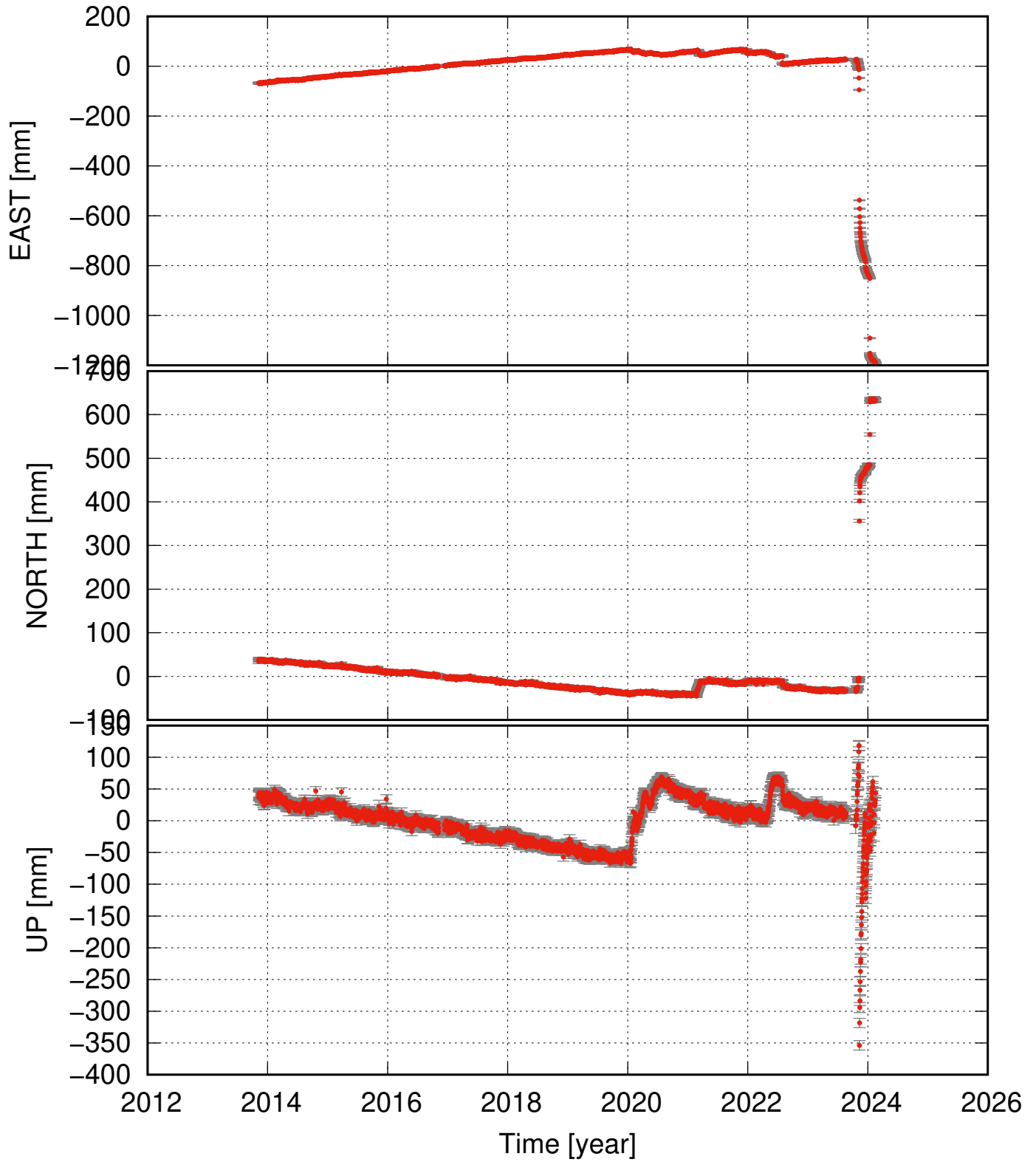
SKSH residual time series (some major events removed as well)
