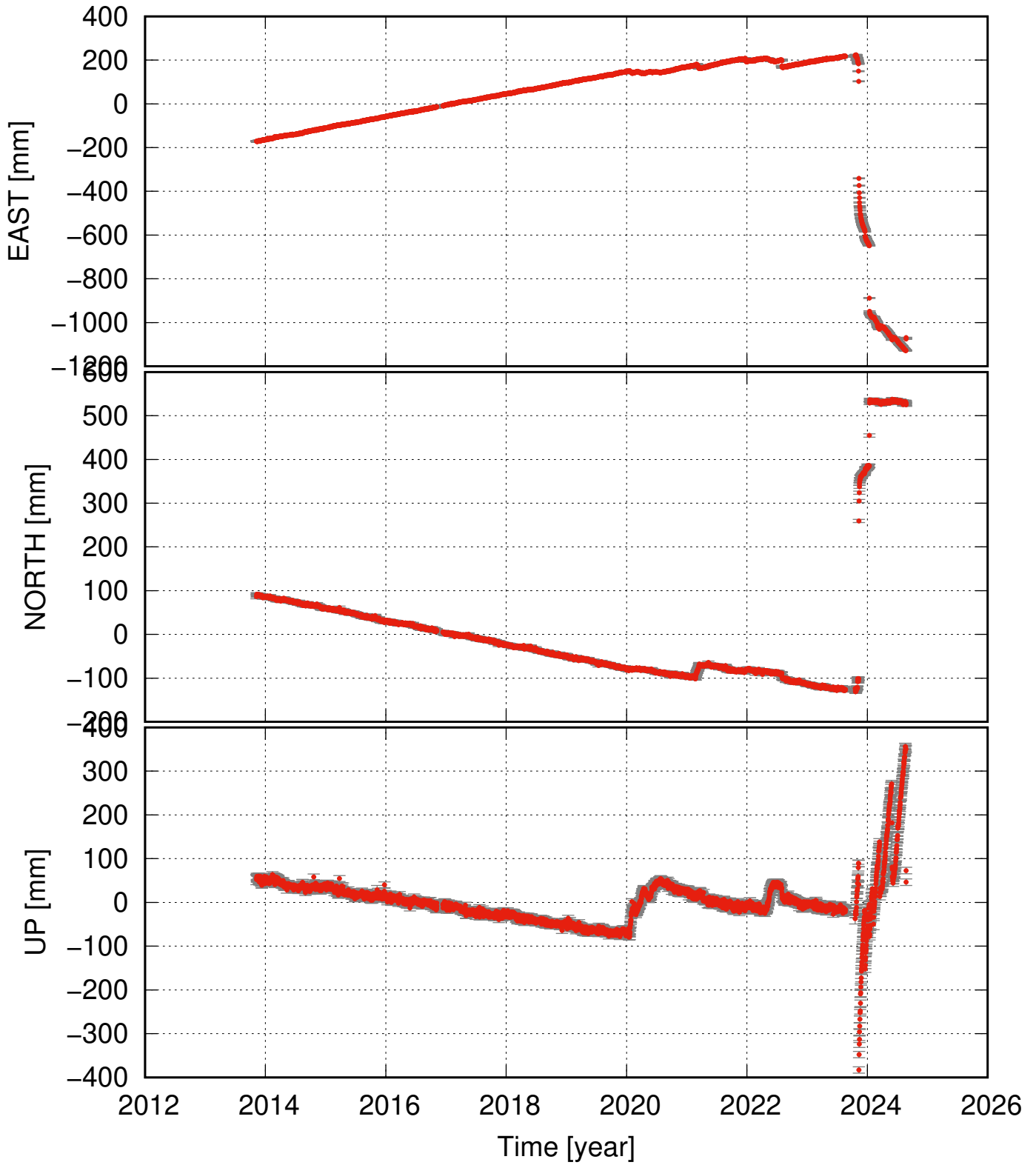
SKSH residual time series
