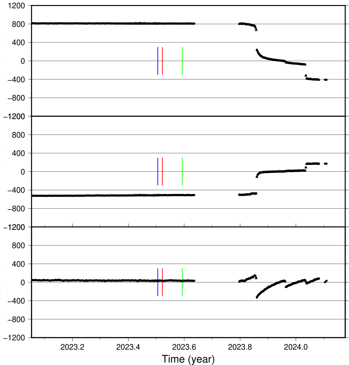
SKSH time series (IGS 2014), last 400 days
