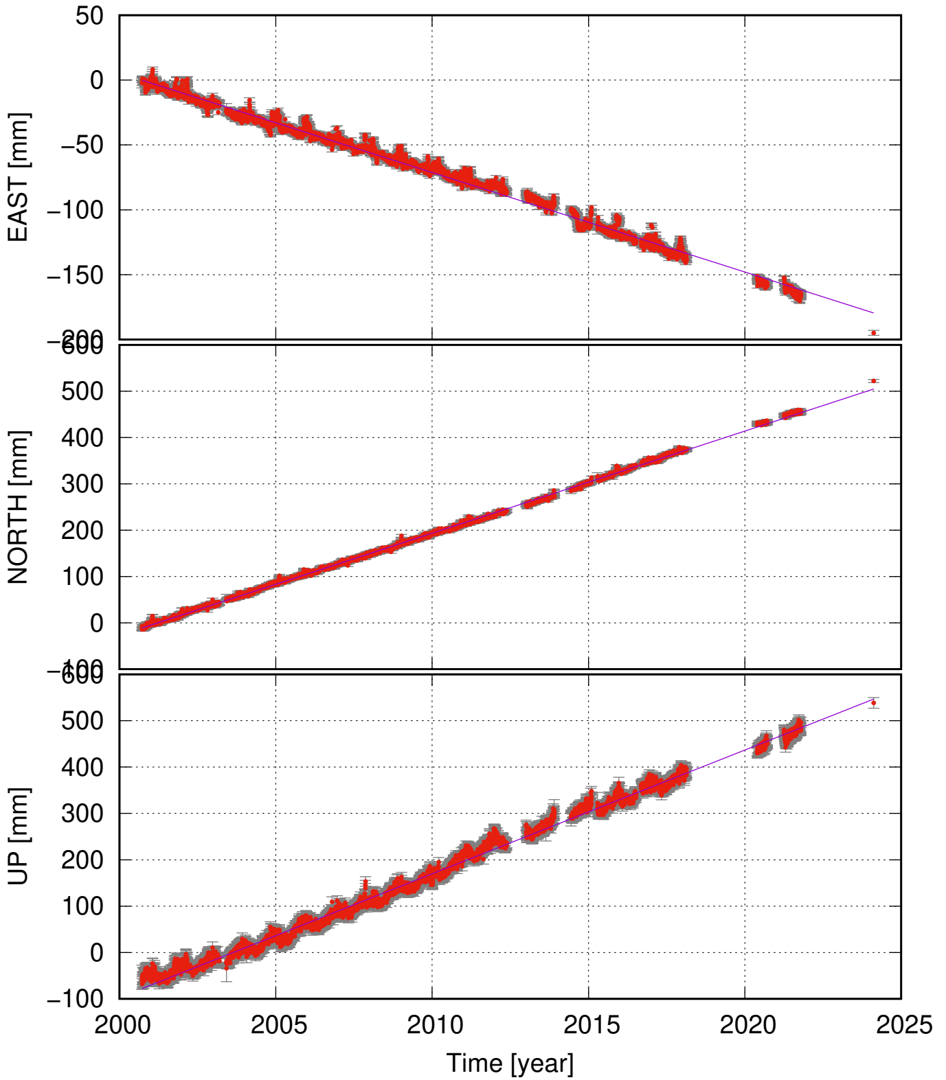
SKRO (64.56, -18.38) time series (ITRF 2014) v_e = -7.67 \pm 0.15 ; v_n = 22.04 \pm 0.14 ; v_u = 26.69 \pm 0.49 mm/yr
