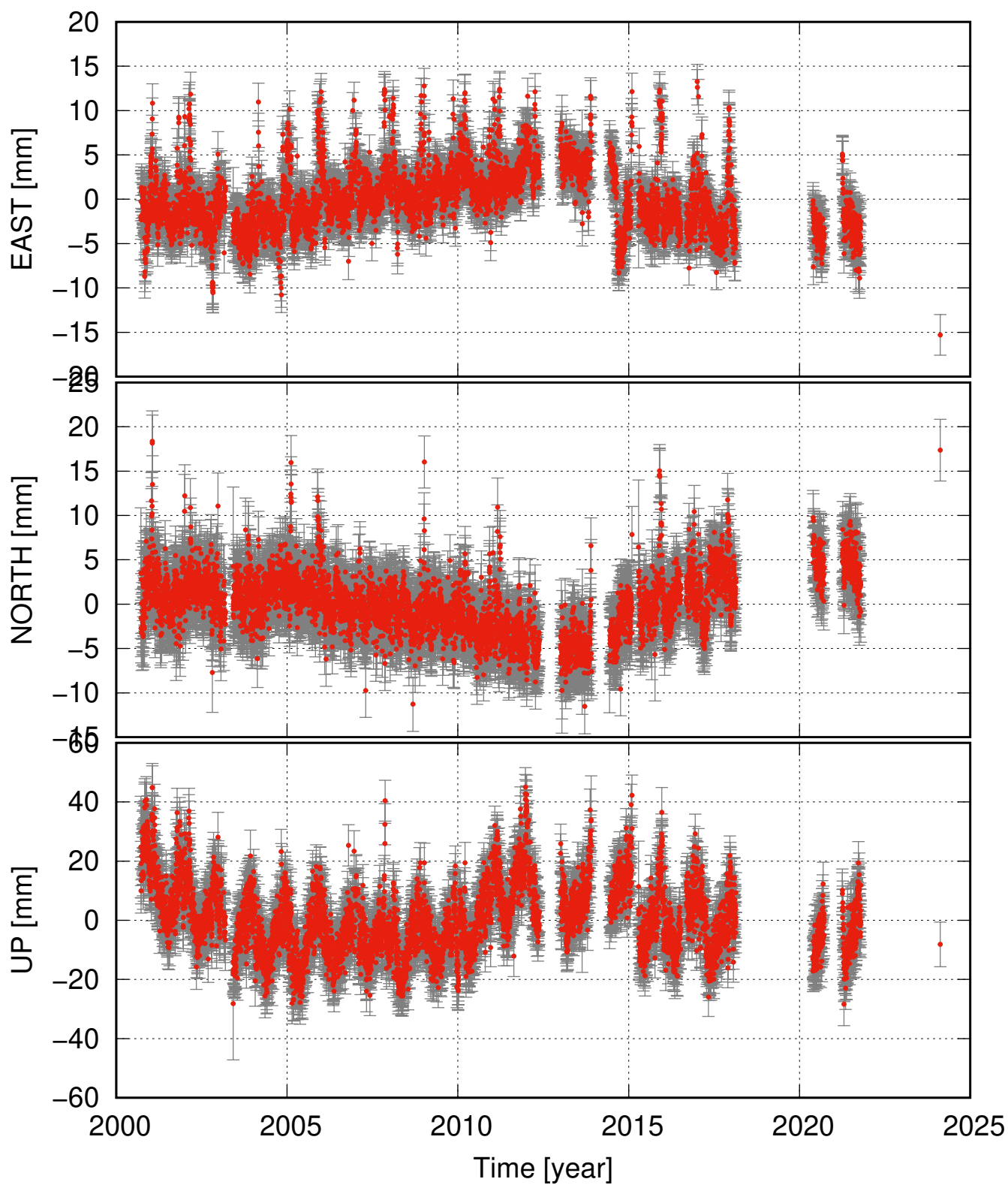
SKRO residual time series (some major events removed as well)
