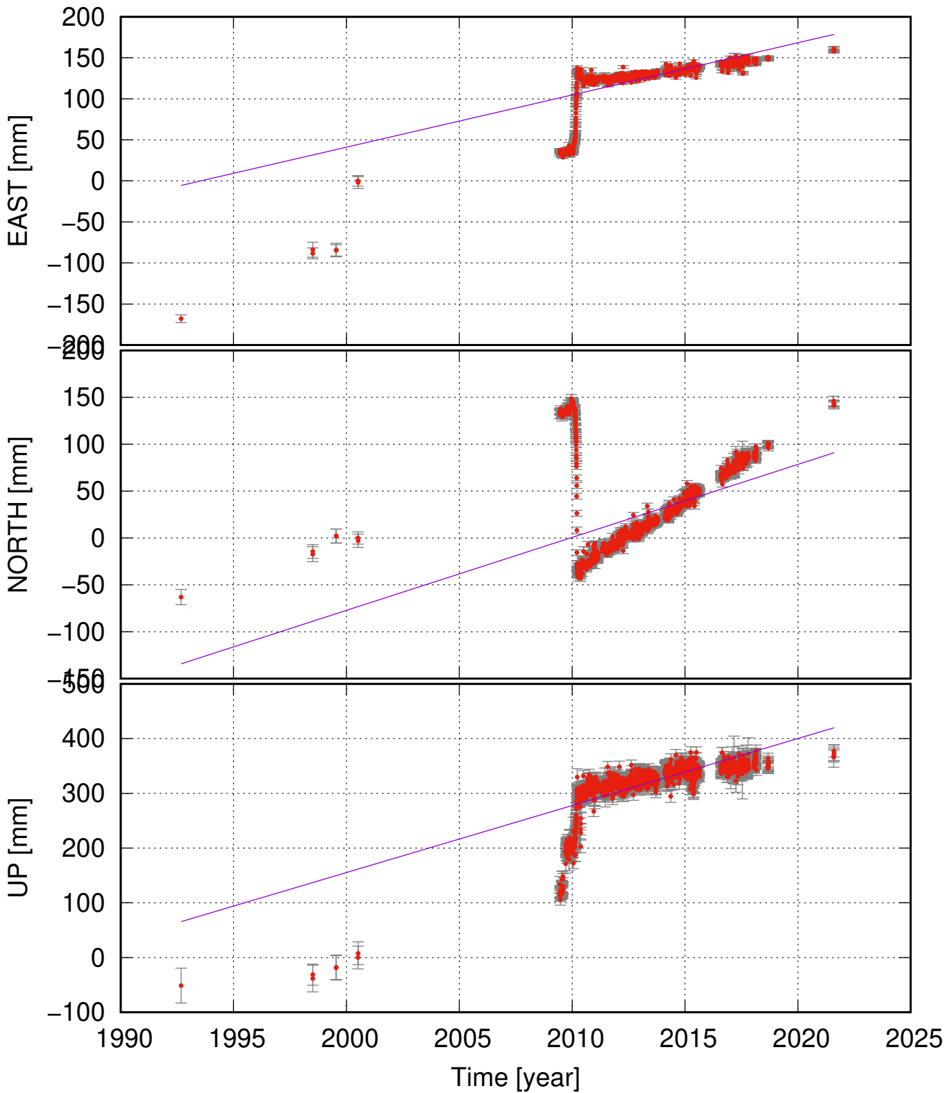
SKOG (63.58, -19.45) time series (ITRF 2014) v_e = 6.36 \pm 0.68 ; v_n = 7.78 \pm 1.41 ; v_u = 12.24 \pm 1.07 mm/yr
