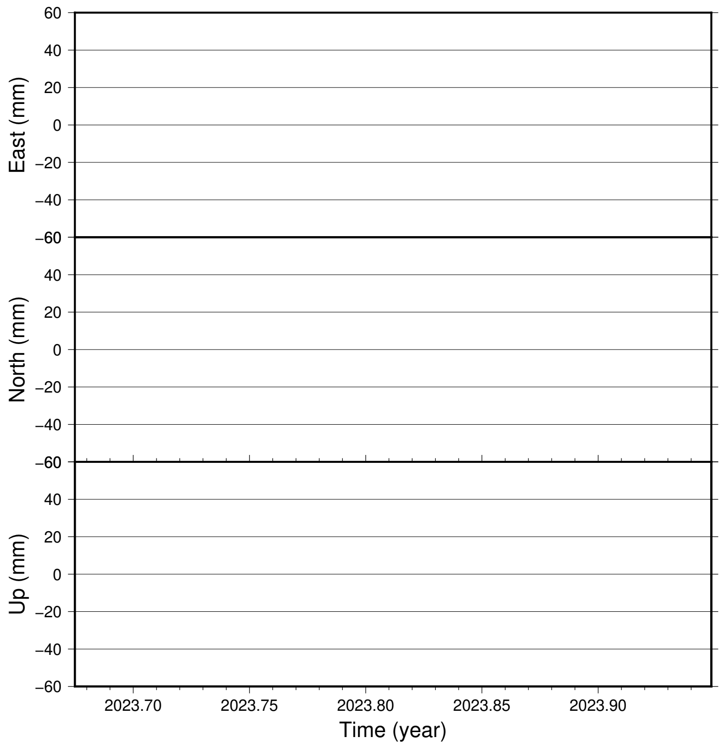
SKOG time series (IGS 2014), last 100 days
