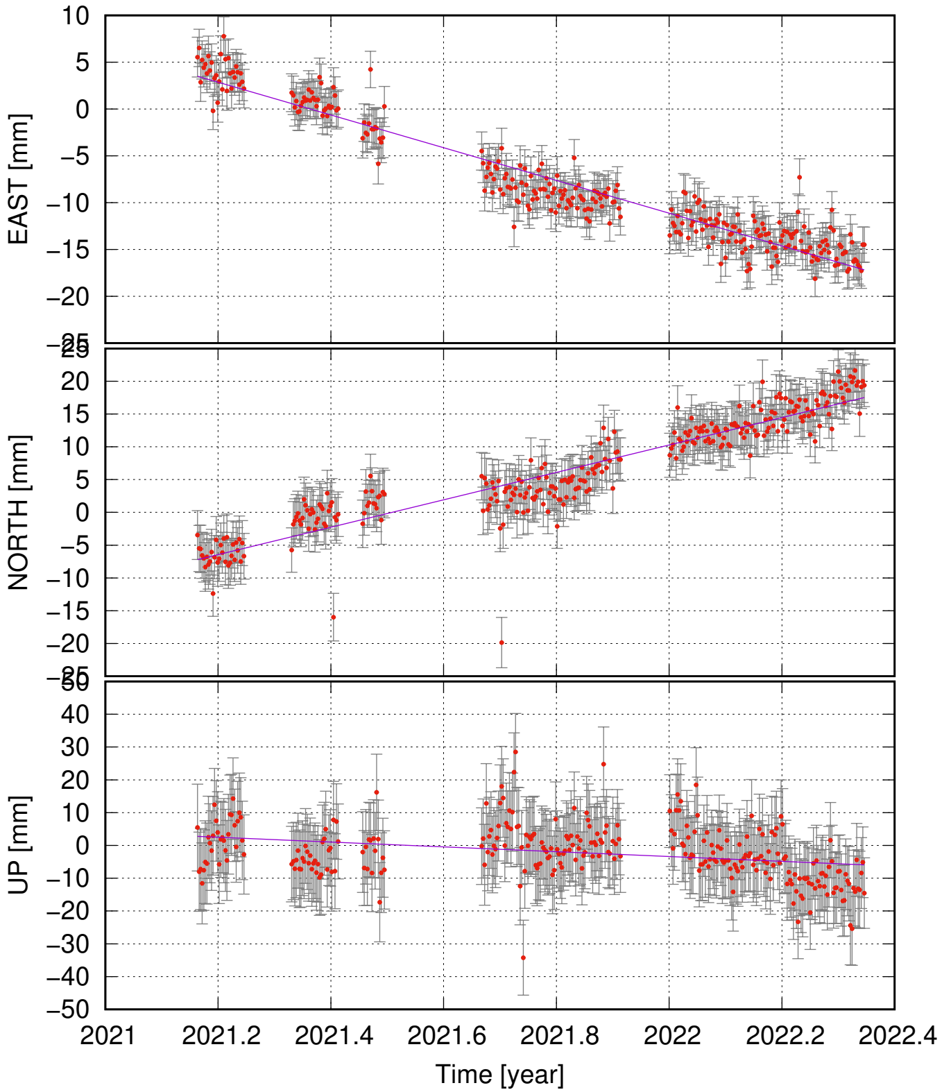
SKHA (64.79, -21.45) time series (ITRF 2014) v_e = -17.49 \pm 1.56 ; v_n = 20.92 \pm 2.46 ; v_u = -7.37 \pm 6.50 mm/yr
