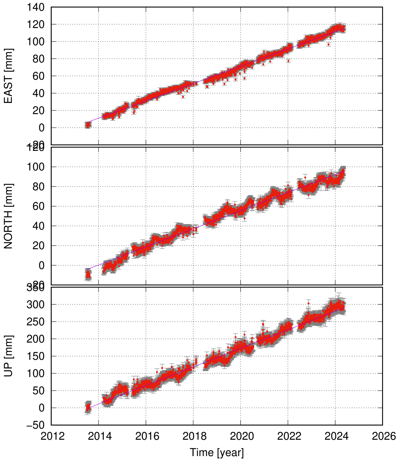
SKFC (64.03, -16.99) time series (ITRF 2014) v_e = 10.04 \pm 0.22 ; v_n = 9.20 \pm 0.35 ; v_u = 26.92 \pm 0.88 mm/yr
