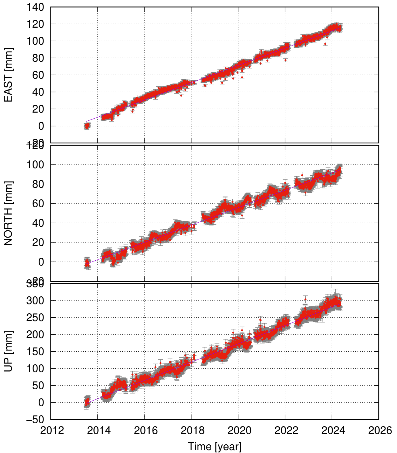
SKFC (64.03, -16.99) time series (ITRF 2014) v_e = 10.15 \pm 0.24 ; v_n = 8.92 \pm 0.32 ; v_u = 26.92 \pm 0.88 mm/yr
