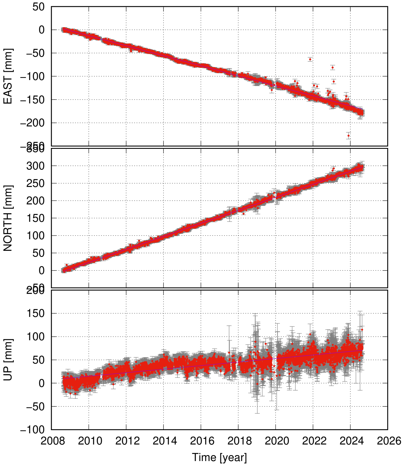
SKDA (64.38, -20.67) time series (ITRF 2014) v_e = -10.78 \pm 0.21 ; v_n = 18.66 \pm 0.18 ; v_u = 3.80 \pm 0.63 mm/yr
