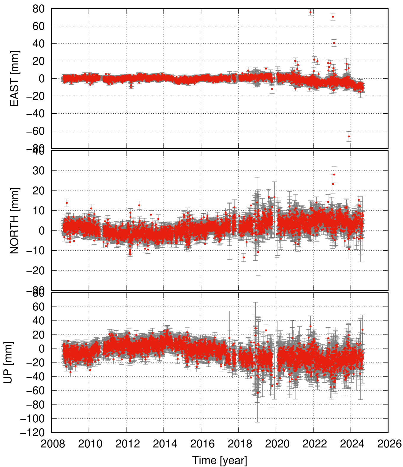
SKDA detrended and seasonal signal removed
