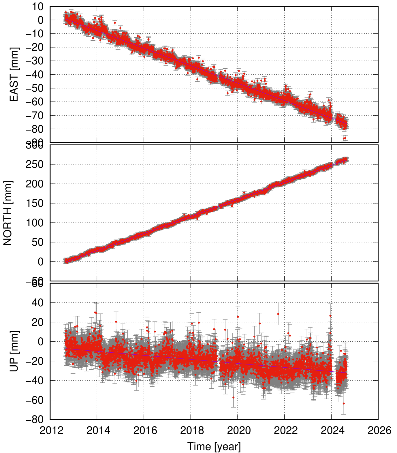
SJUK (66.05, -17.34) time series (ITRF 2014) v_e = -6.41 \pm 0.18 ; v_n = 21.90 \pm 0.20 ; v_u = -2.08 \pm 0.63 mm/yr
