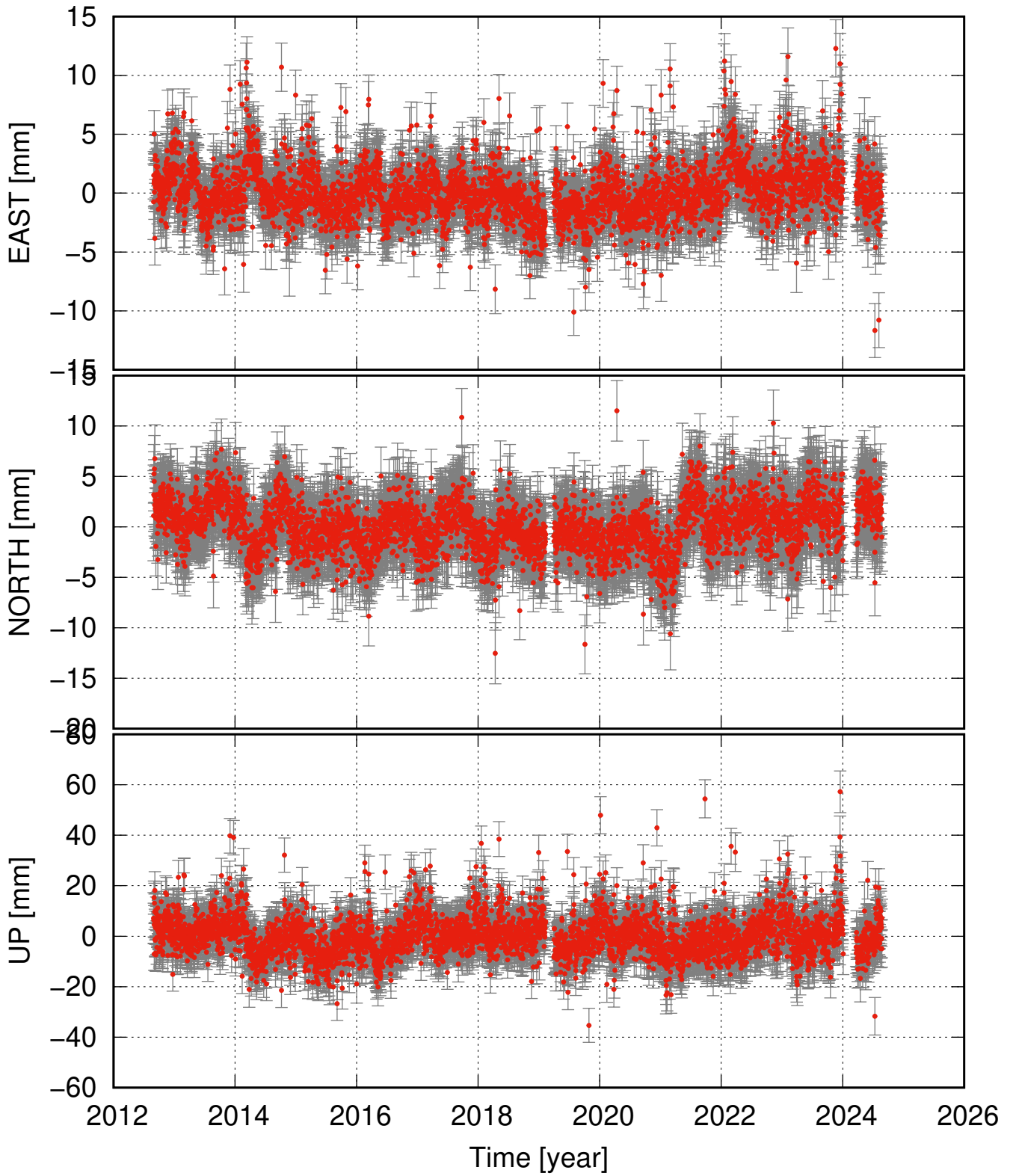
SJUK residual time series (some major events removed as well)
