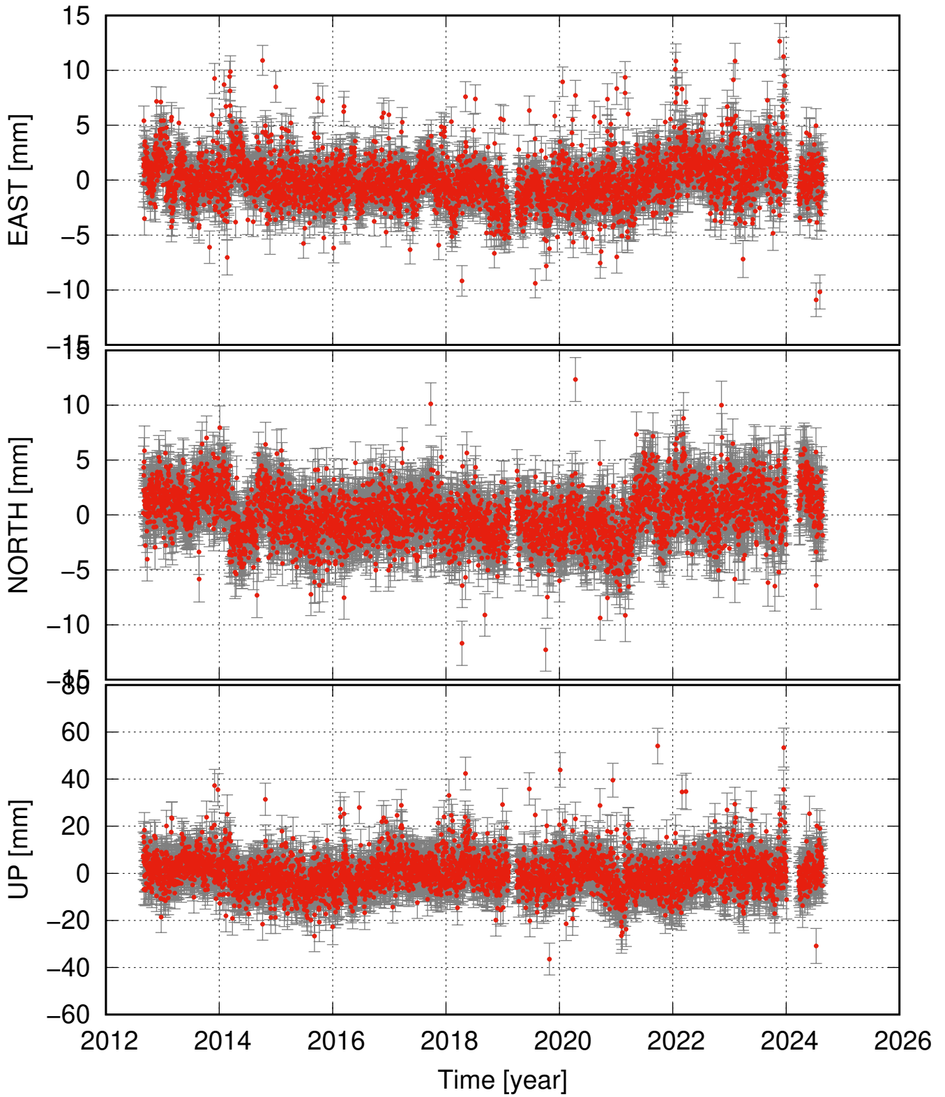
SJUK detrended and seasonal signal removed
