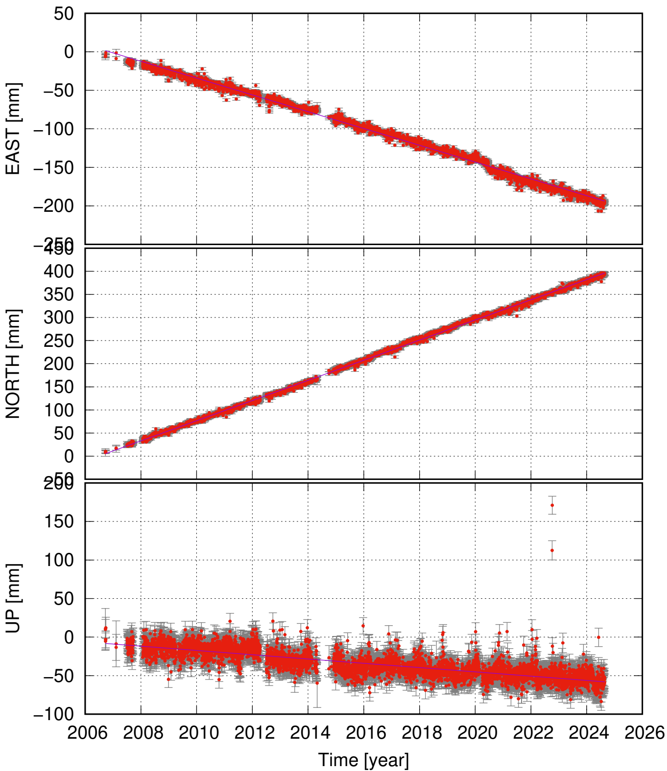
SIFJ (66.14, -18.90) time series (ITRF 2014) v_e = -10.90 \pm 0.21 ; v_n = 21.81 \pm 0.18 ; v_u = -2.78 \pm 0.56 mm/yr
