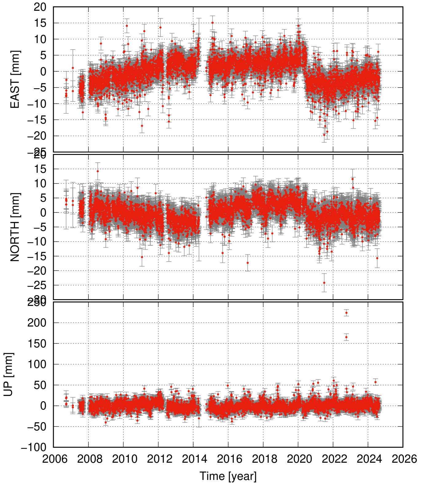
SIFJ residual time series (some major events removed as well)
