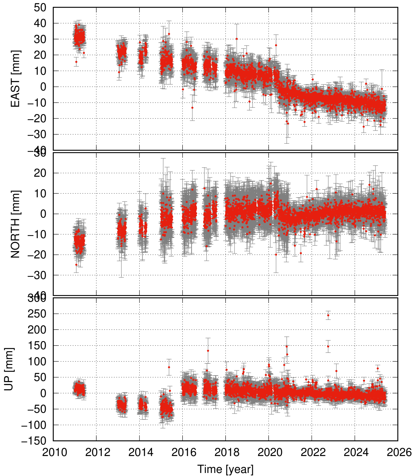
SIFJ time series relative to the NA plate
