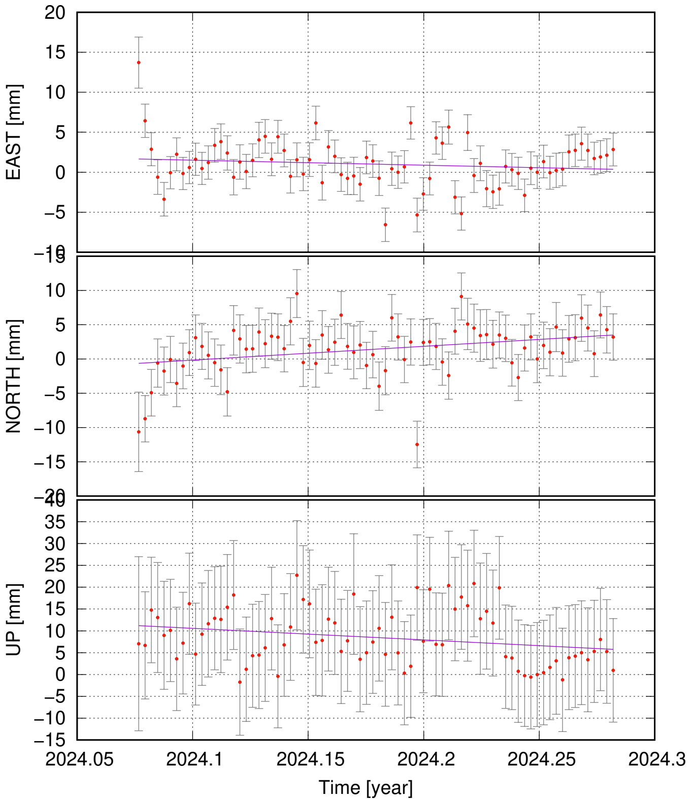
SEY9 (65.26, -13.99) time series (ITRF 2014) v_e = -6.28 \pm 14.35 ; v_n = 20.15 \pm 16.97 ; v_u = -26.43 \pm 30.07 mm/yr
