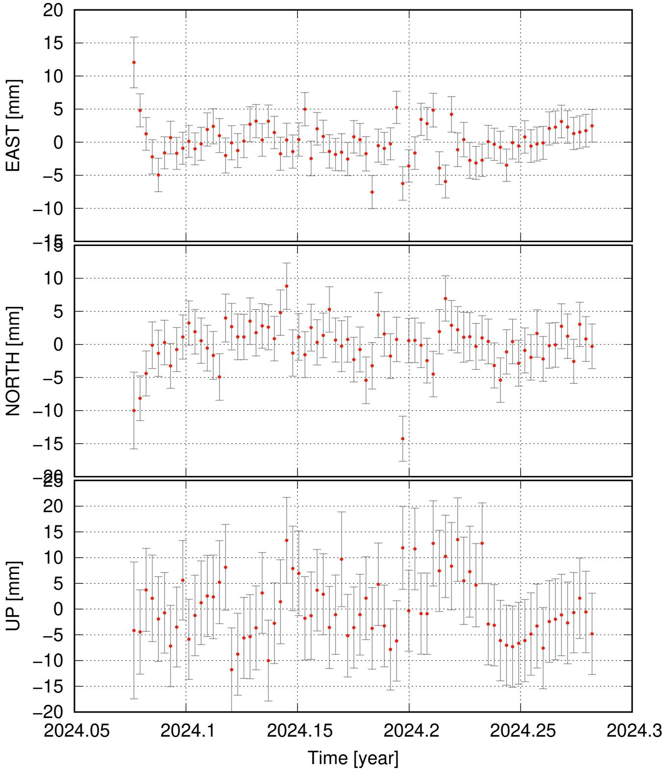
SEY9 residual time series (some major events removed as well)
