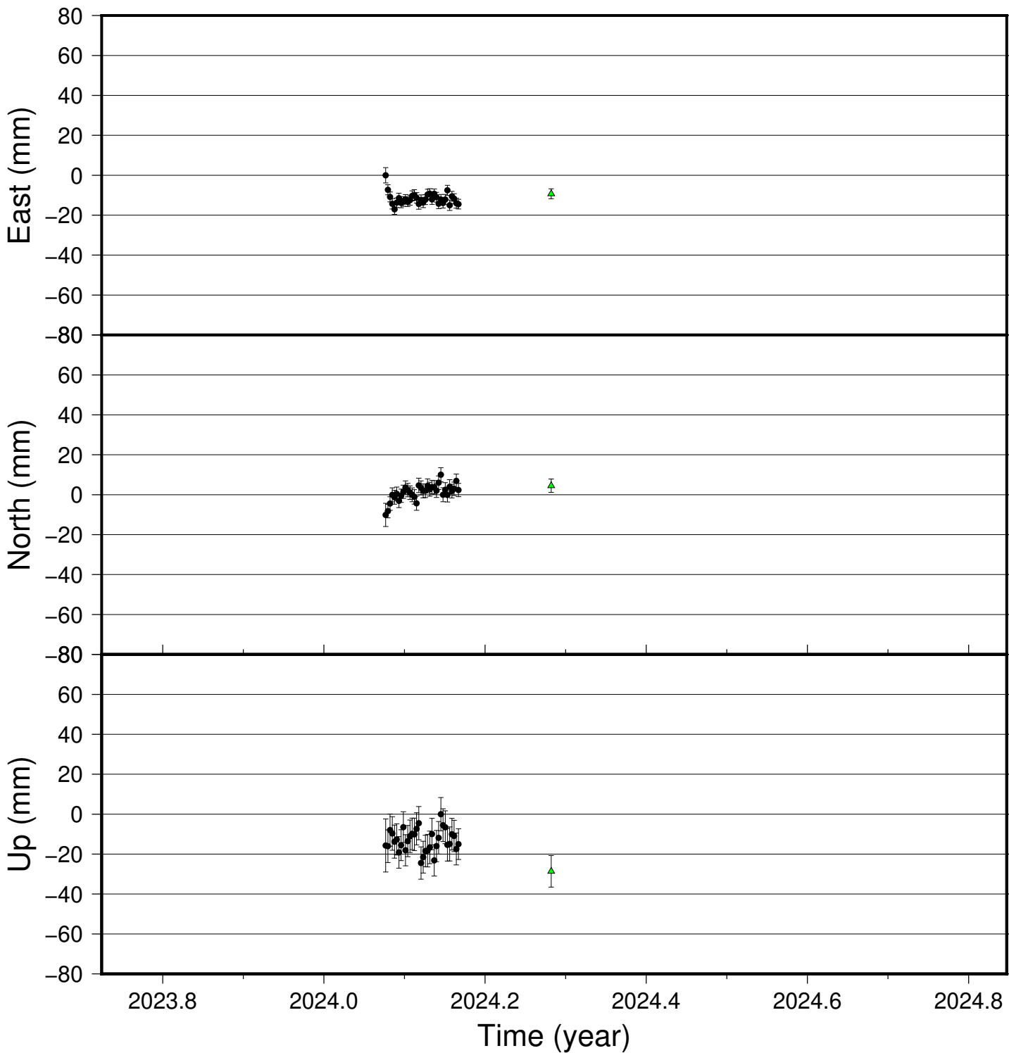
SEY9 time series (IGS 2014), last 400 days
