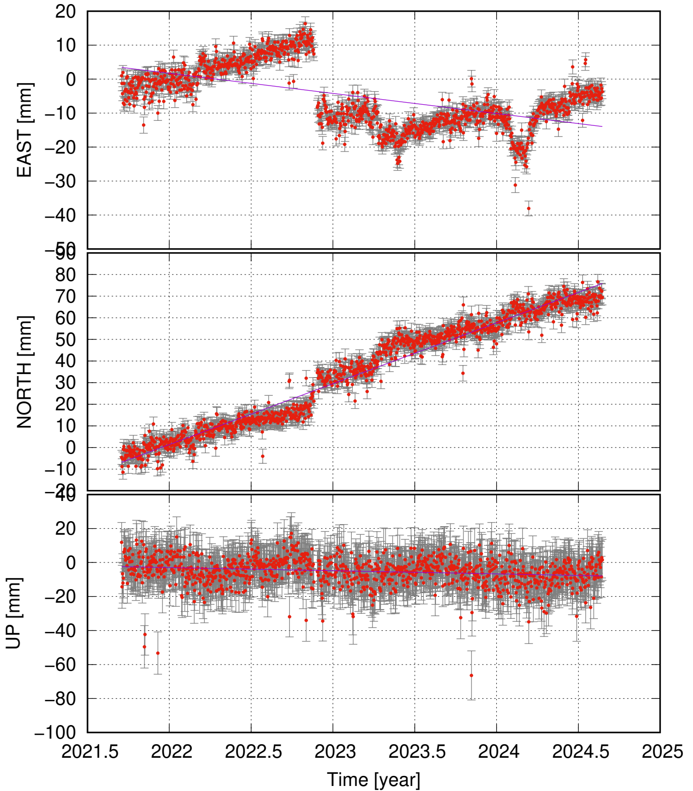
SEY8 (65.26, -13.99) time series (ITRF 2014) v_e = -5.93 \pm 2.52 ; v_n = 28.16 \pm 1.64 ; v_u = -1.84 \pm 2.75 mm/yr
