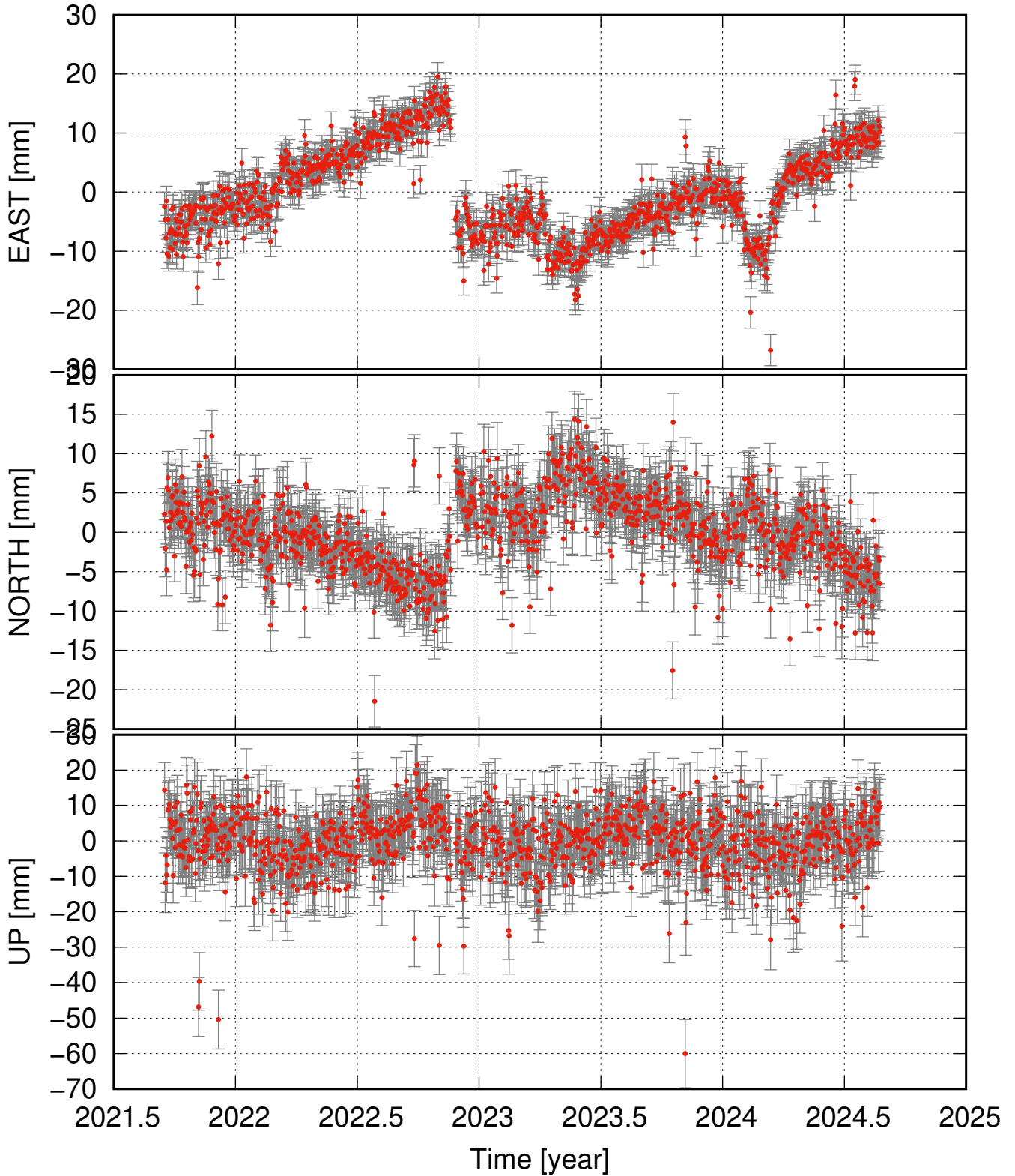
SEY8 residual time series (some major events removed as well)
