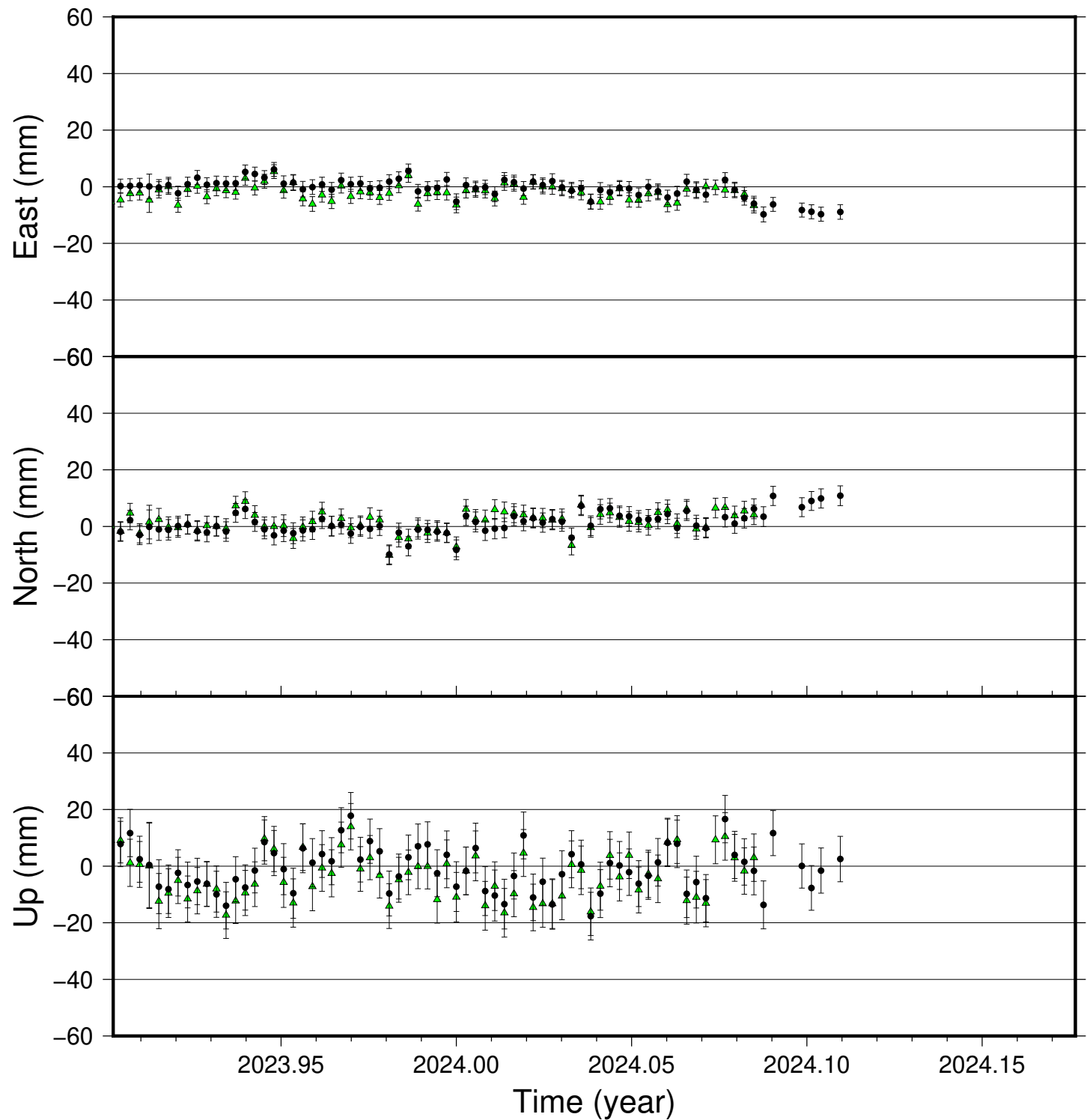
SEY8 time series (IGS 2014), last 100 days
