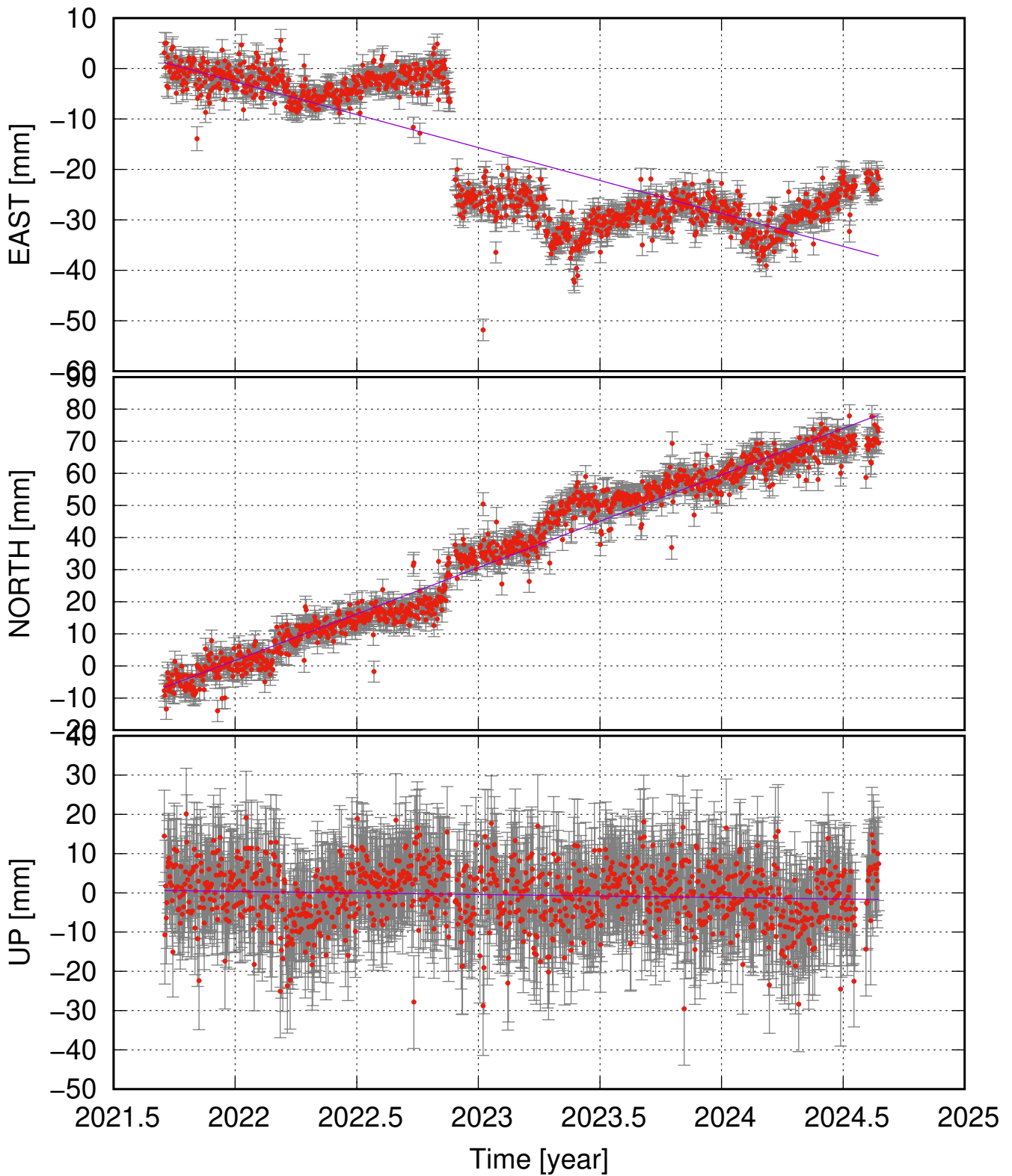
SEY7 (65.26, -13.99) time series (ITRF 2014) v_e = -13.04 \pm 2.55 ; v_n = 28.90 \pm 1.60 ; v_u = -0.77 \pm 2.53 mm/yr
